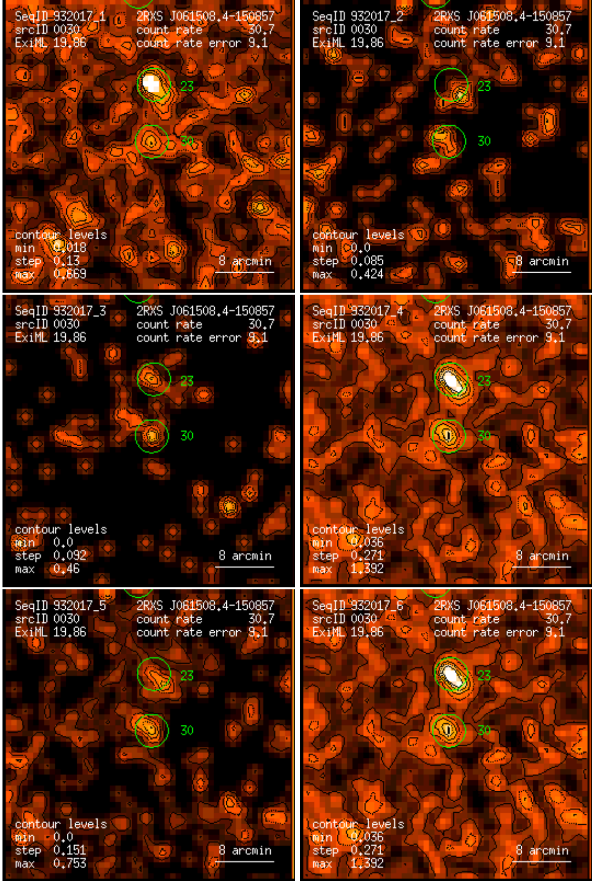
Figure 30: RASS 932017: detection 0030: band rate images, Gaussian filter: (1) PSPC channels 11 – 41, (2) 52 – 90, (3) 91 – 201, (4) 11 – 235, (5) 52 – 201, (6) 11 – 201. Broad band rates in counts/ks. Band rate contour levels in counts/ks/arcmin 2 .
