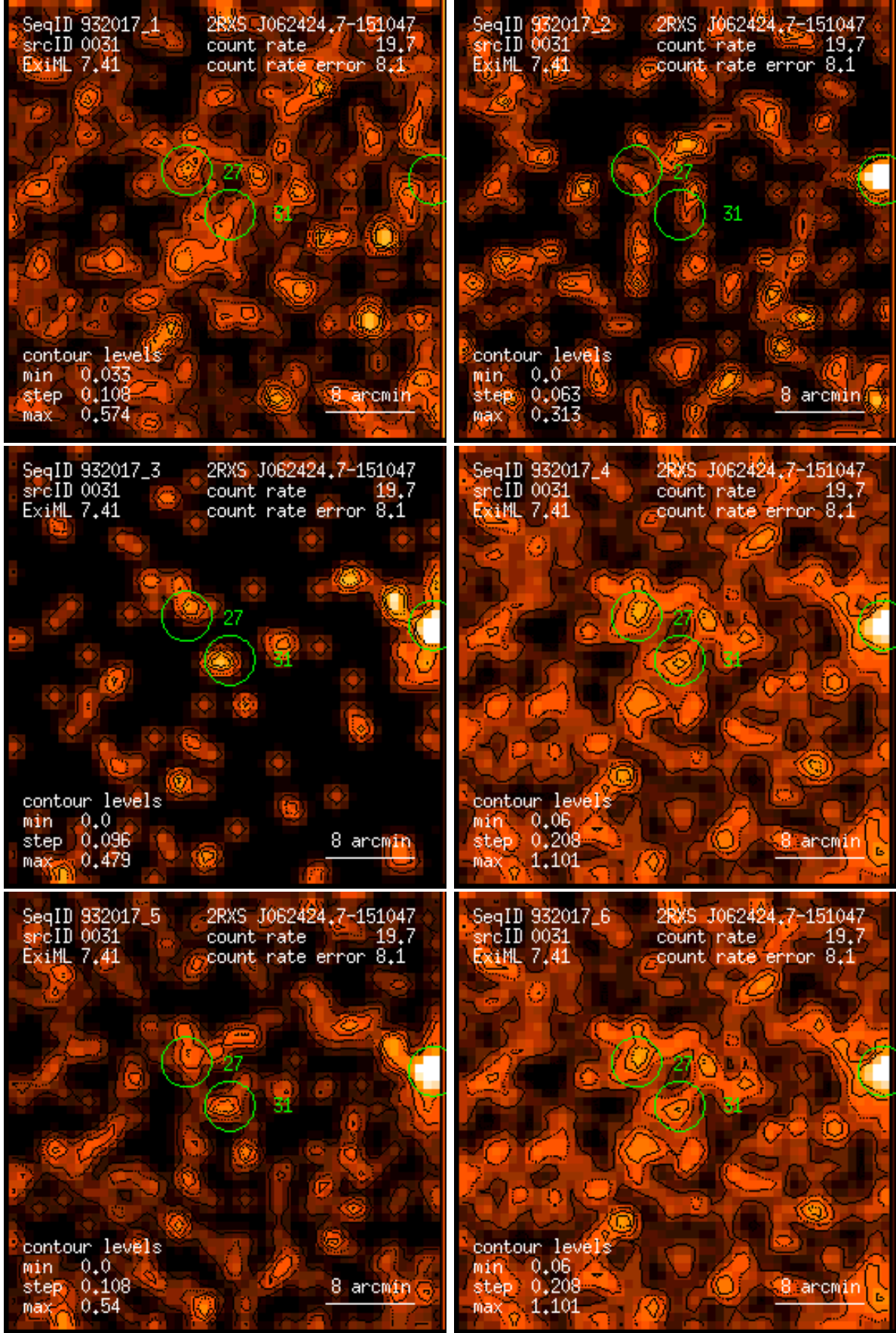
Figure 31: RASS 932017: detection 0031: band rate images, Gaussian filter: (1) PSPC channels 11 – 41, (2) 52 – 90, (3) 91 – 201, (4) 11 – 235, (5) 52 – 201, (6) 11 – 201. Broad band rates in counts/ks. Band rate contour levels in counts/ks/arcmin 2 .
