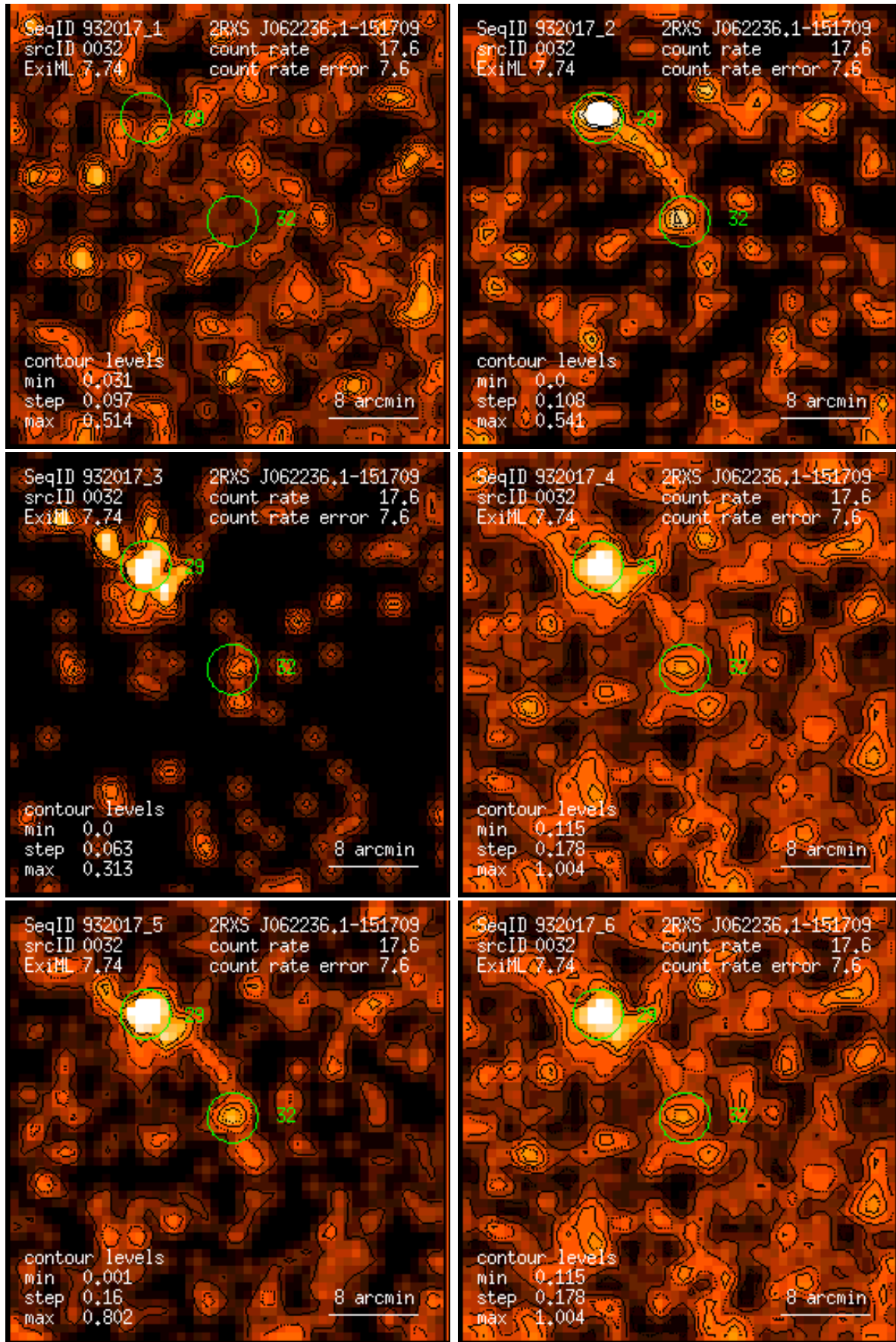
Figure 32: RASS 932017: detection 0032: band rate images, Gaussian filter: (1) PSPC channels 11 – 41, (2) 52 – 90, (3) 91 – 201, (4) 11 – 235, (5) 52 – 201, (6) 11 – 201. Broad band rates in counts/ks. Band rate contour levels in counts/ks/arcmin 2 .
