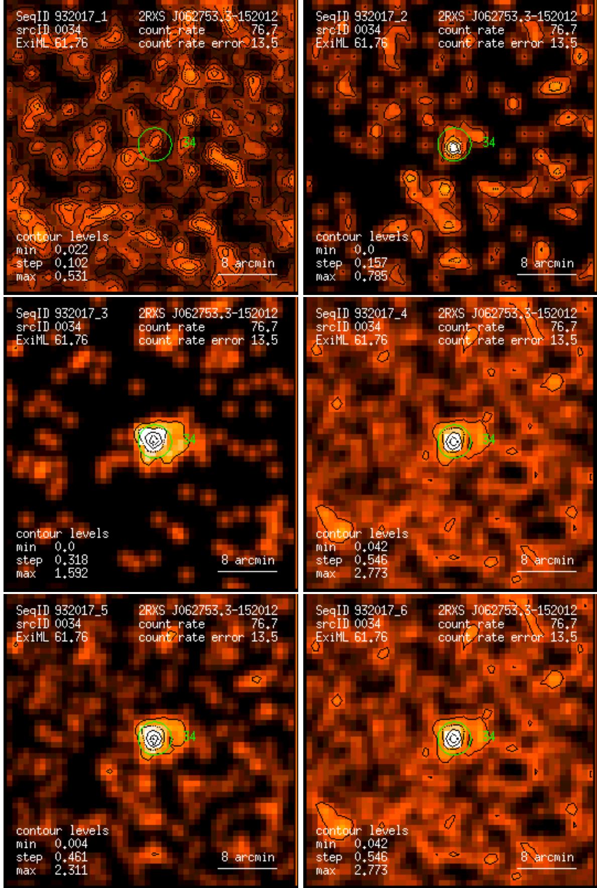
Figure 34: RASS 932017: detection 0034: band rate images, Gaussian filter: (1) PSPC channels 11 – 41, (2) 52 – 90, (3) 91 – 201, (4) 11 – 235, (5) 52 – 201, (6) 11 – 201. Broad band rates in counts/ks. Band rate contour levels in counts/ks/arcmin 2 .
