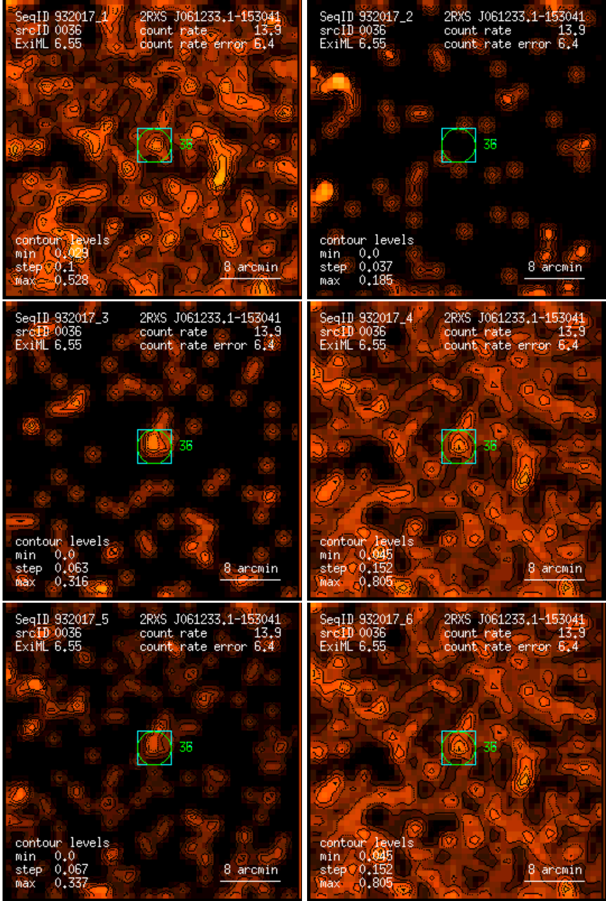
Figure 36: RASS 932017: detection 0036: band rate images, Gaussian filter: (1) PSPC channels 11 – 41, (2) 52 – 90, (3) 91 – 201, (4) 11 – 235, (5) 52 – 201, (6) 11 – 201. Broad band rates in counts/ks. Band rate contour levels in counts/ks/arcmin 2 .
