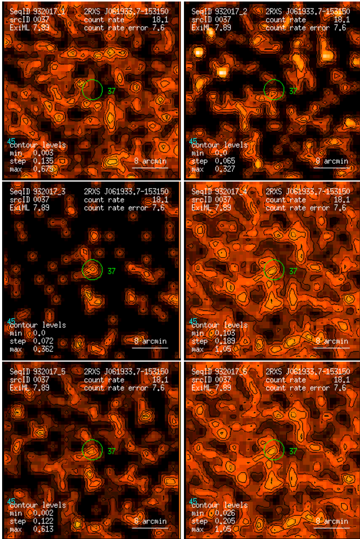
Figure 37: RASS 932017: detection 0037: band rate images, Gaussian filter: (1) PSPC channels 11 – 41, (2) 52 – 90, (3) 91 – 201, (4) 11 – 235, (5) 52 – 201, (6) 11 – 201. Broad band rates in counts/ks. Band rate contour levels in counts/ks/arcmin 2 .
