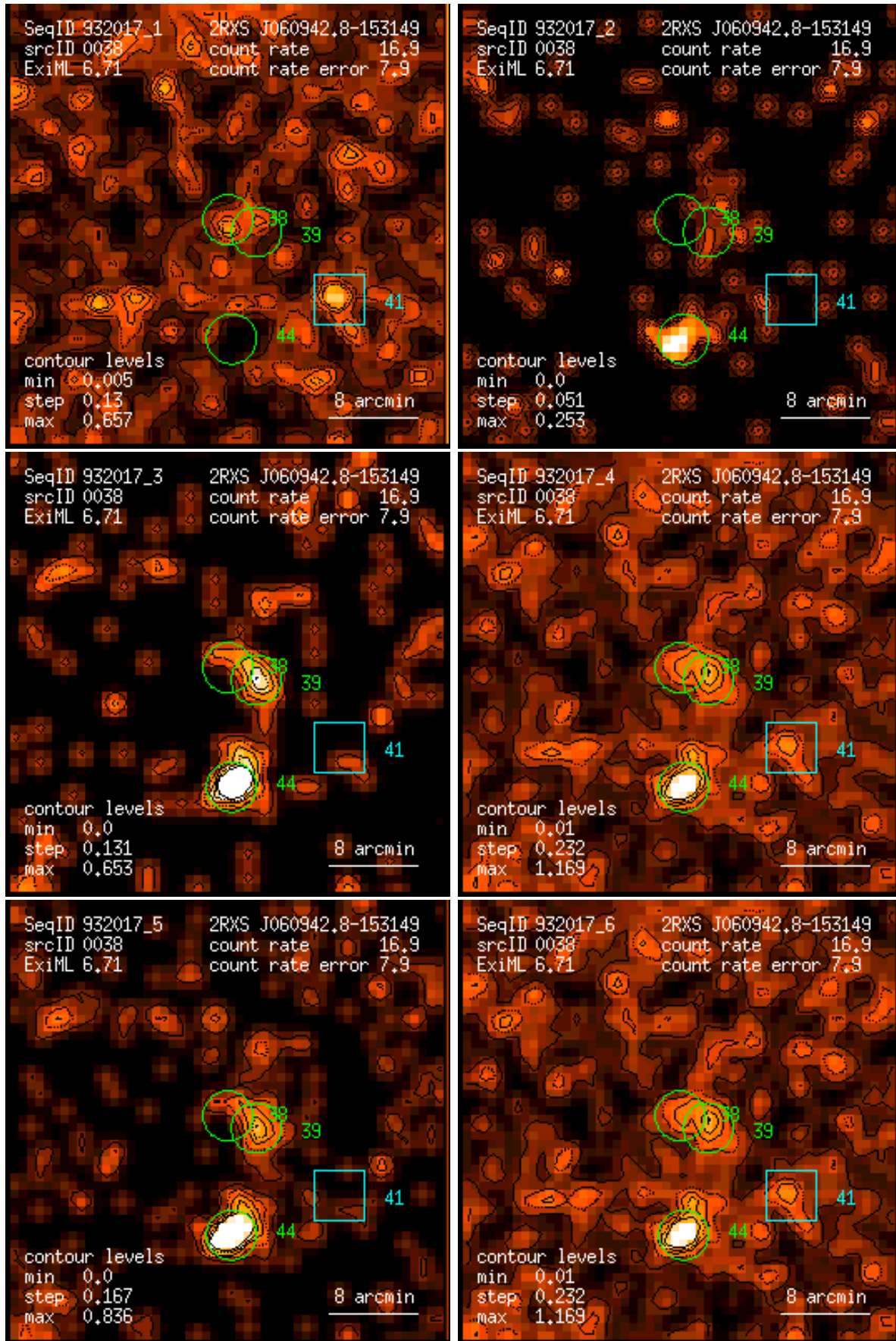
Figure 38: RASS 932017: detection 0038: band rate images, Gaussian filter: (1) PSPC channels 11 – 41, (2) 52 – 90, (3) 91 – 201, (4) 11 – 235, (5) 52 – 201, (6) 11 – 201. Broad band rates in counts/ks. Band rate contour levels in counts/ks/arcmin 2 .
