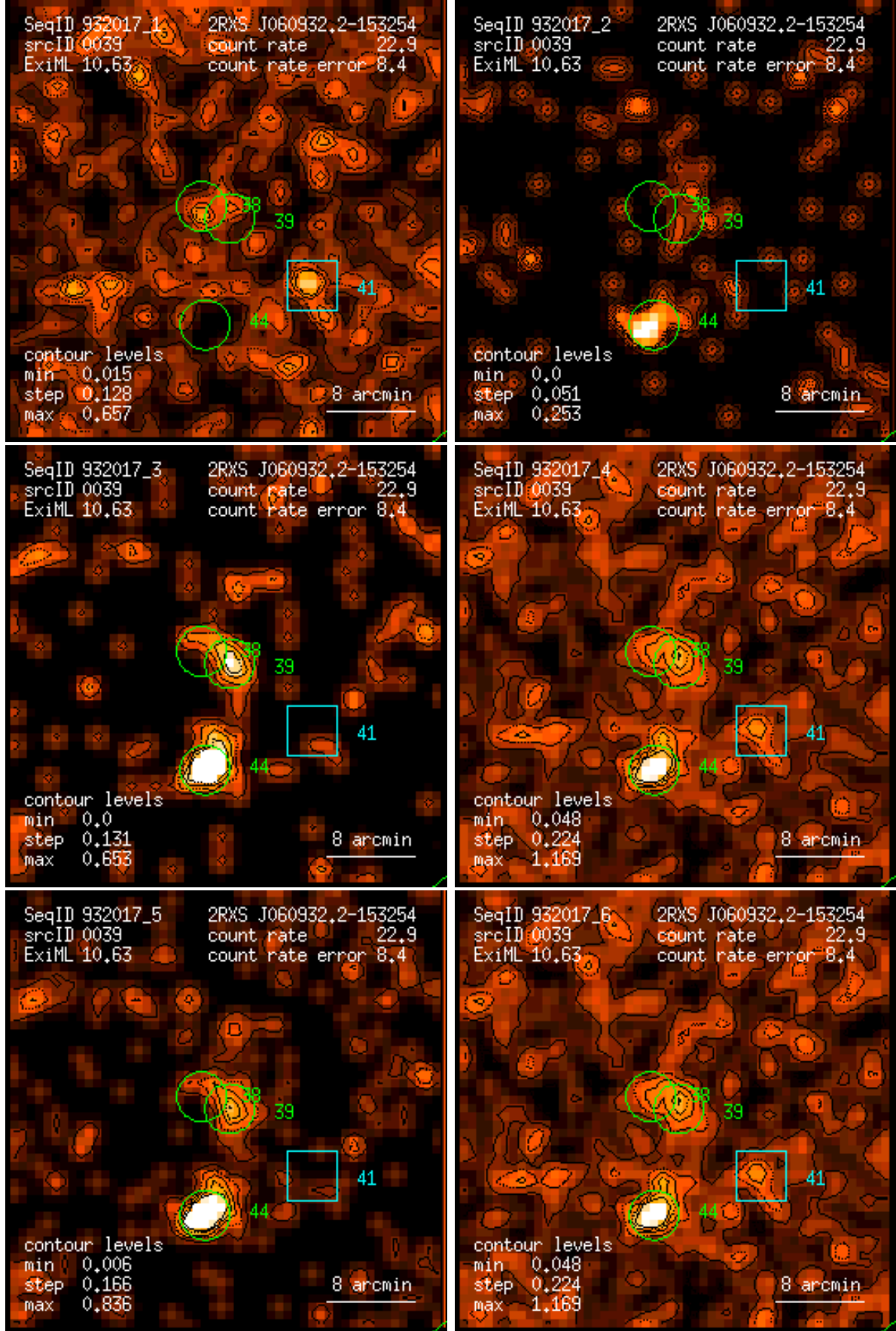
Figure 39: RASS 932017: detection 0039: band rate images, Gaussian filter: (1) PSPC channels 11 – 41, (2) 52 – 90, (3) 91 – 201, (4) 11 – 235, (5) 52 – 201, (6) 11 – 201. Broad band rates in counts/ks. Band rate contour levels in counts/ks/arcmin 2 .
