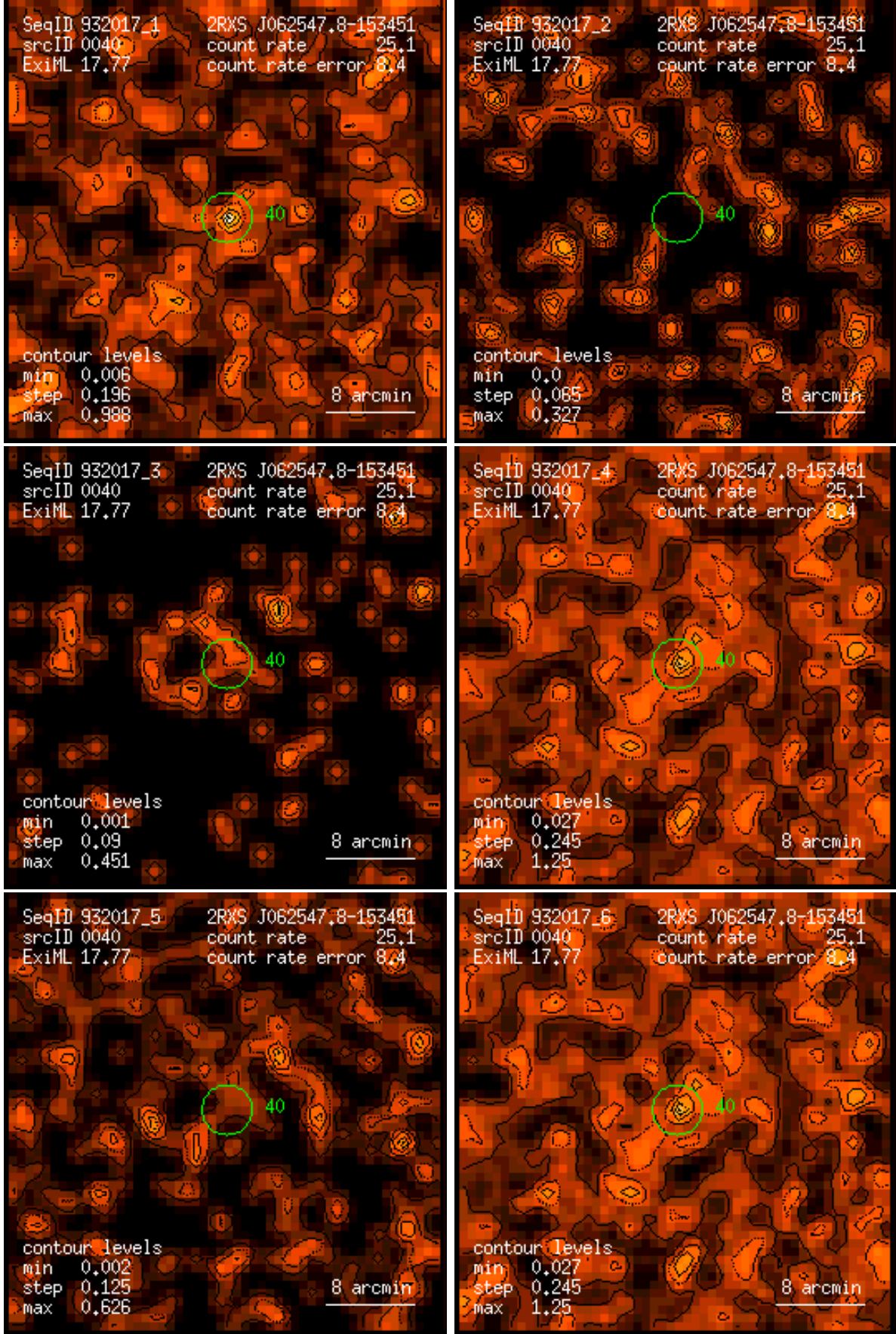
Figure 40: RASS 932017: detection 0040: band rate images, Gaussian filter: (1) PSPC channels 11 – 41, (2) 52 – 90, (3) 91 – 201, (4) 11 – 235, (5) 52 – 201, (6) 11 – 201. Broad band rates in counts/ks. Band rate contour levels in counts/ks/arcmin 2 .
