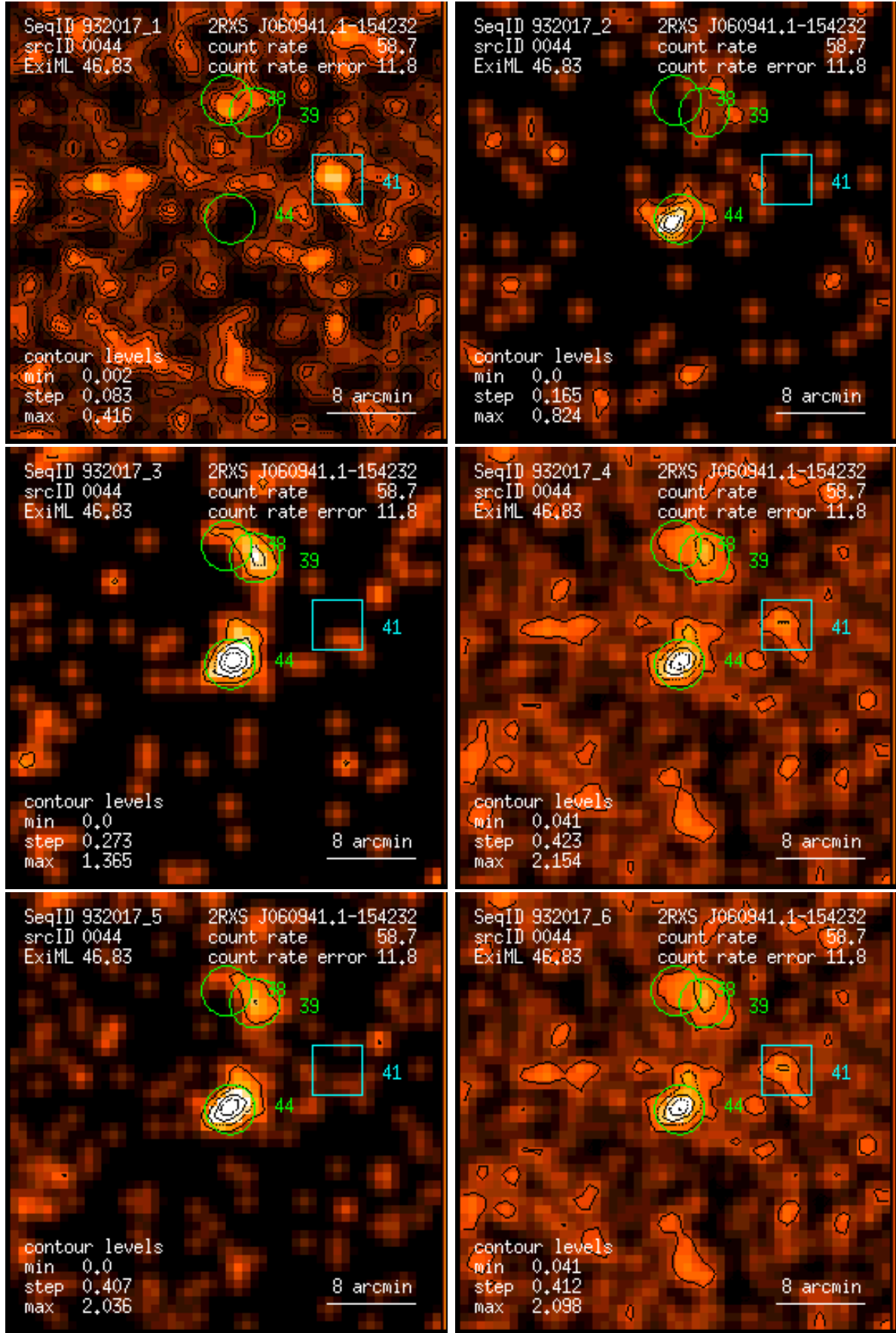
Figure 44: RASS 932017: detection 0044: band rate images, Gaussian filter: (1) PSPC channels 11 – 41, (2) 52 – 90, (3) 91 – 201, (4) 11 – 235, (5) 52 – 201, (6) 11 – 201. Broad band rates in counts/ks. Band rate contour levels in counts/ks/arcmin 2 .
