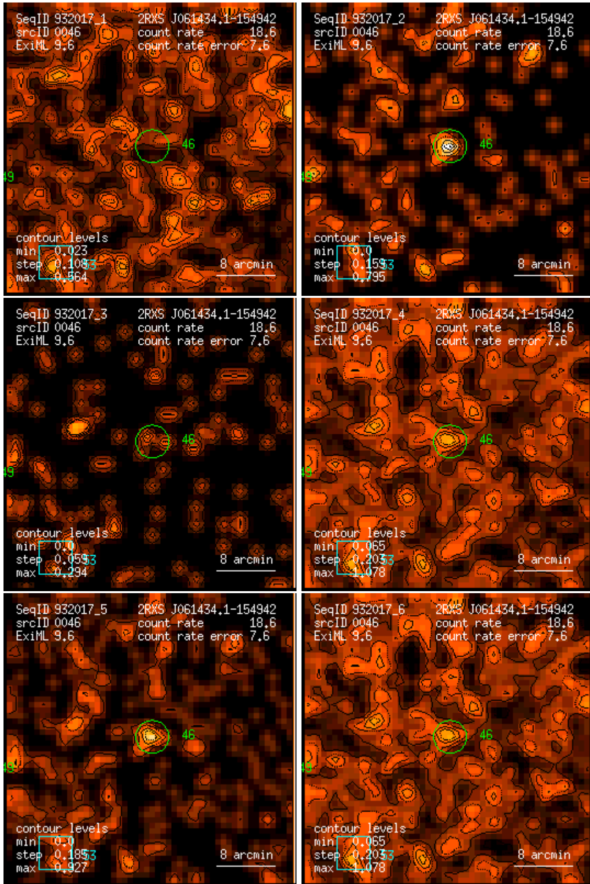
Figure 46: RASS 932017: detection 0046: band rate images, Gaussian filter: (1) PSPC channels 11 – 41, (2) 52 – 90, (3) 91 – 201, (4) 11 – 235, (5) 52 – 201, (6) 11 – 201. Broad band rates in counts/ks. Band rate contour levels in counts/ks/arcmin 2 .
