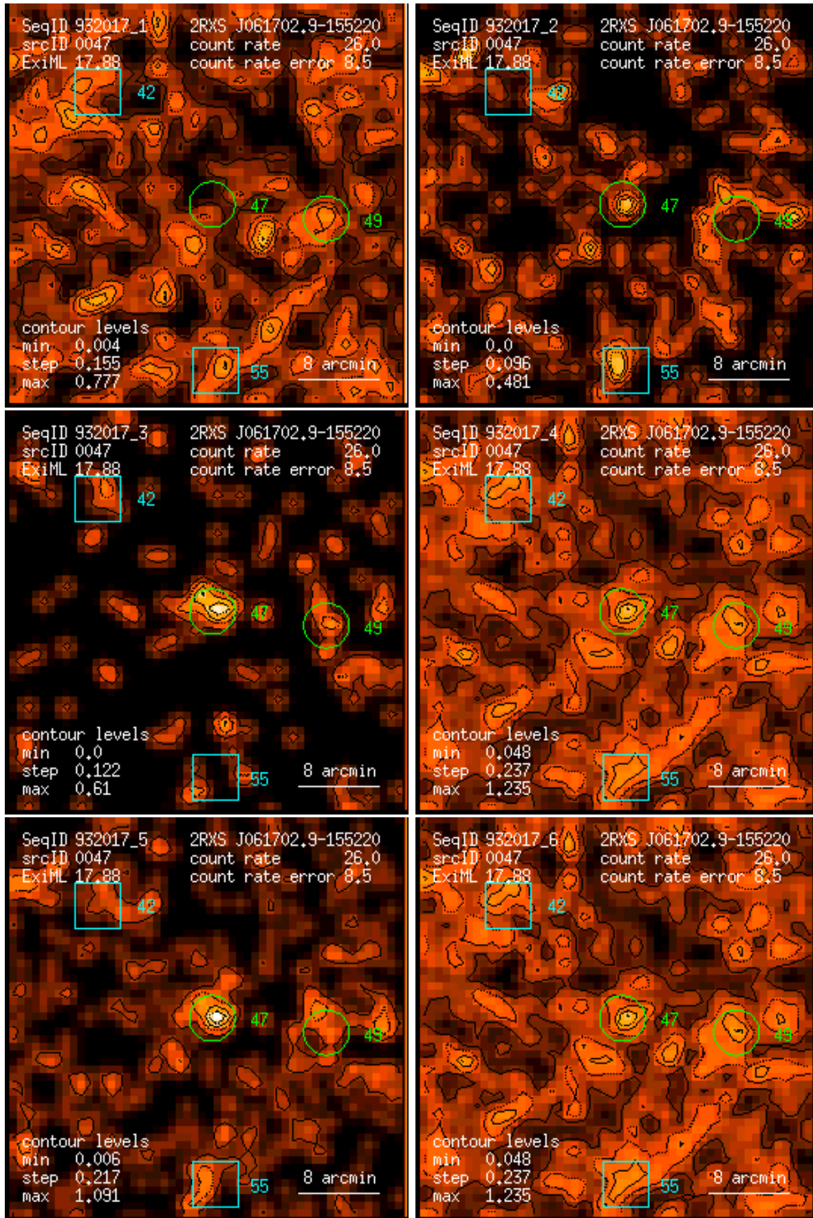
Figure 47: RASS 932017: detection 0047: band rate images, Gaussian filter: (1) PSPC channels 11 – 41, (2) 52 – 90, (3) 91 – 201, (4) 11 – 235, (5) 52 – 201, (6) 11 – 201. Broad band rates in counts/ks. Band rate contour levels in counts/ks/arcmin 2 .
