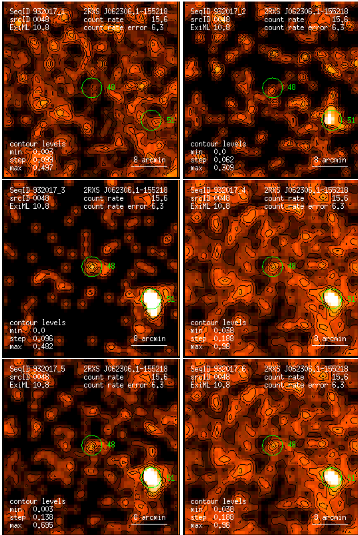
Figure 48: RASS 932017: detection 0048: band rate images, Gaussian filter: (1) PSPC channels 11 – 41, (2) 52 – 90, (3) 91 – 201, (4) 11 – 235, (5) 52 – 201, (6) 11 – 201. Broad band rates in counts/ks. Band rate contour levels in counts/ks/arcmin 2 .
