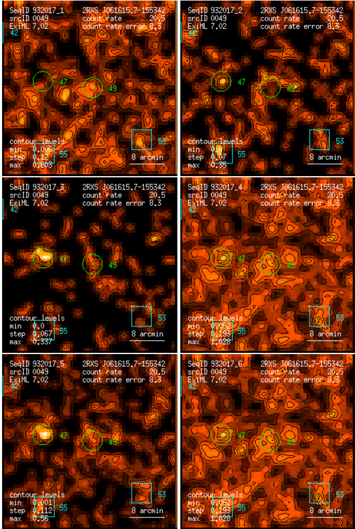
Figure 49: RASS 932017: detection 0049: band rate images, Gaussian filter: (1) PSPC channels 11 – 41, (2) 52 – 90, (3) 91 – 201, (4) 11 – 235, (5) 52 – 201, (6) 11 – 201. Broad band rates in counts/ks. Band rate contour levels in counts/ks/arcmin 2 .
