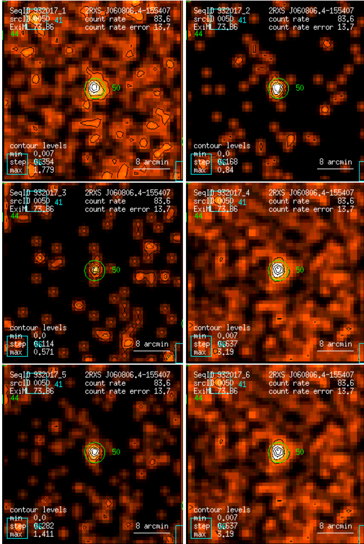
Figure 50: RASS 932017: detection 0050: band rate images, Gaussian filter: (1) PSPC channels 11 – 41, (2) 52 – 90, (3) 91 – 201, (4) 11 – 235, (5) 52 – 201, (6) 11 – 201. Broad band rates in counts/ks. Band rate contour levels in counts/ks/arcmin 2 .
