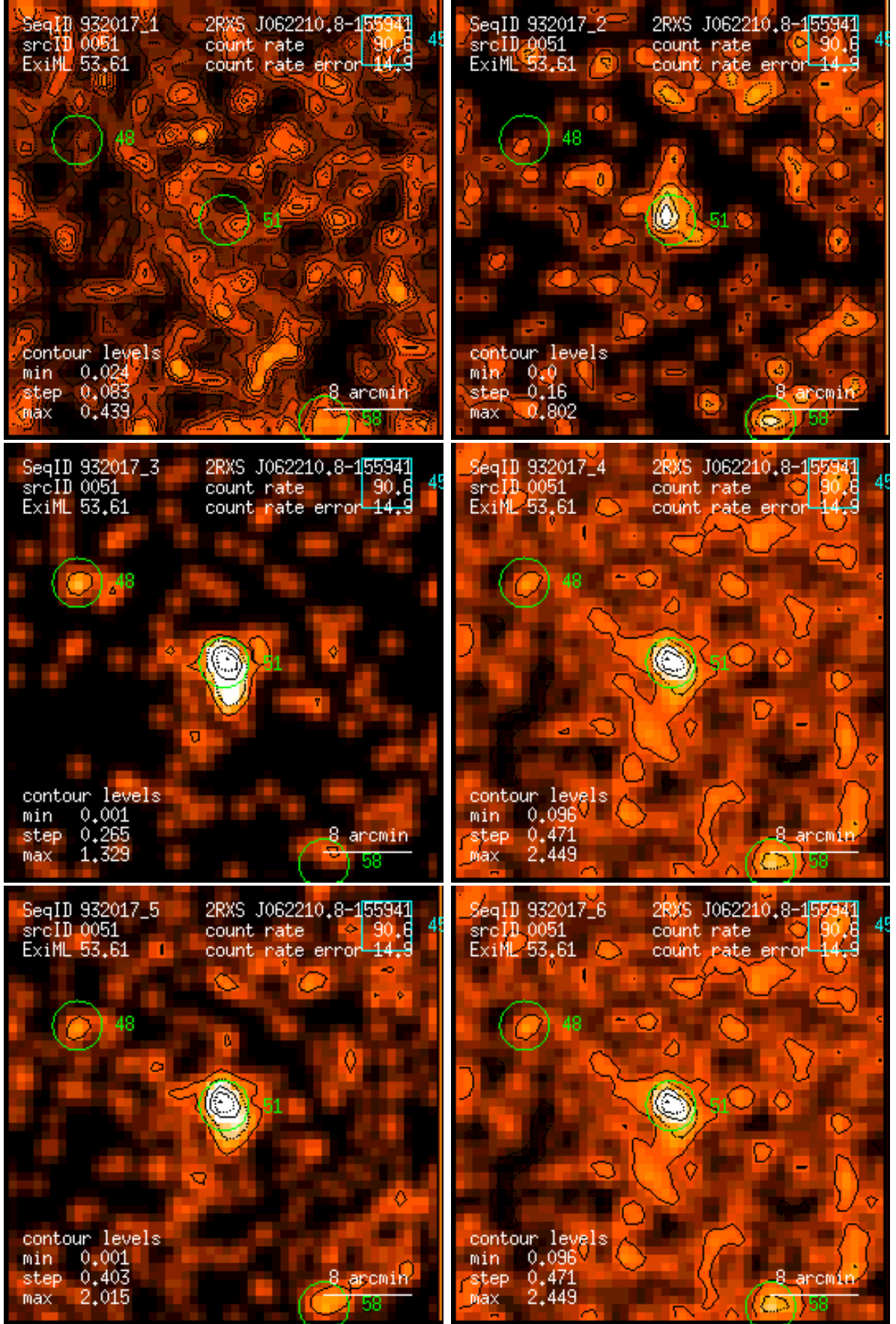
Figure 51: RASS 932017: detection 0051: band rate images, Gaussian filter: (1) PSPC channels 11 – 41, (2) 52 – 90, (3) 91 – 201, (4) 11 – 235, (5) 52 – 201, (6) 11 – 201. Broad band rates in counts/ks. Band rate contour levels in counts/ks/arcmin 2 .
