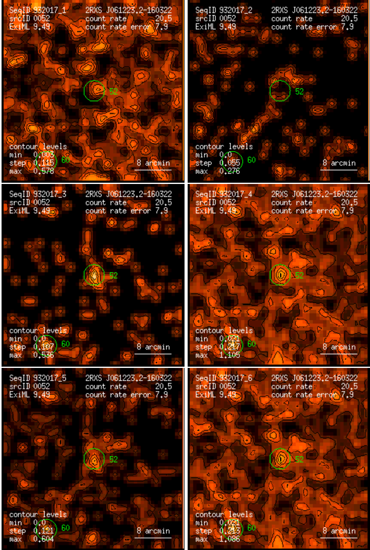
Figure 52: RASS 932017: detection 0052: band rate images, Gaussian filter: (1) PSPC channels 11 – 41, (2) 52 – 90, (3) 91 – 201, (4) 11 – 235, (5) 52 – 201, (6) 11 – 201. Broad band rates in counts/ks. Band rate contour levels in counts/ks/arcmin 2 .
