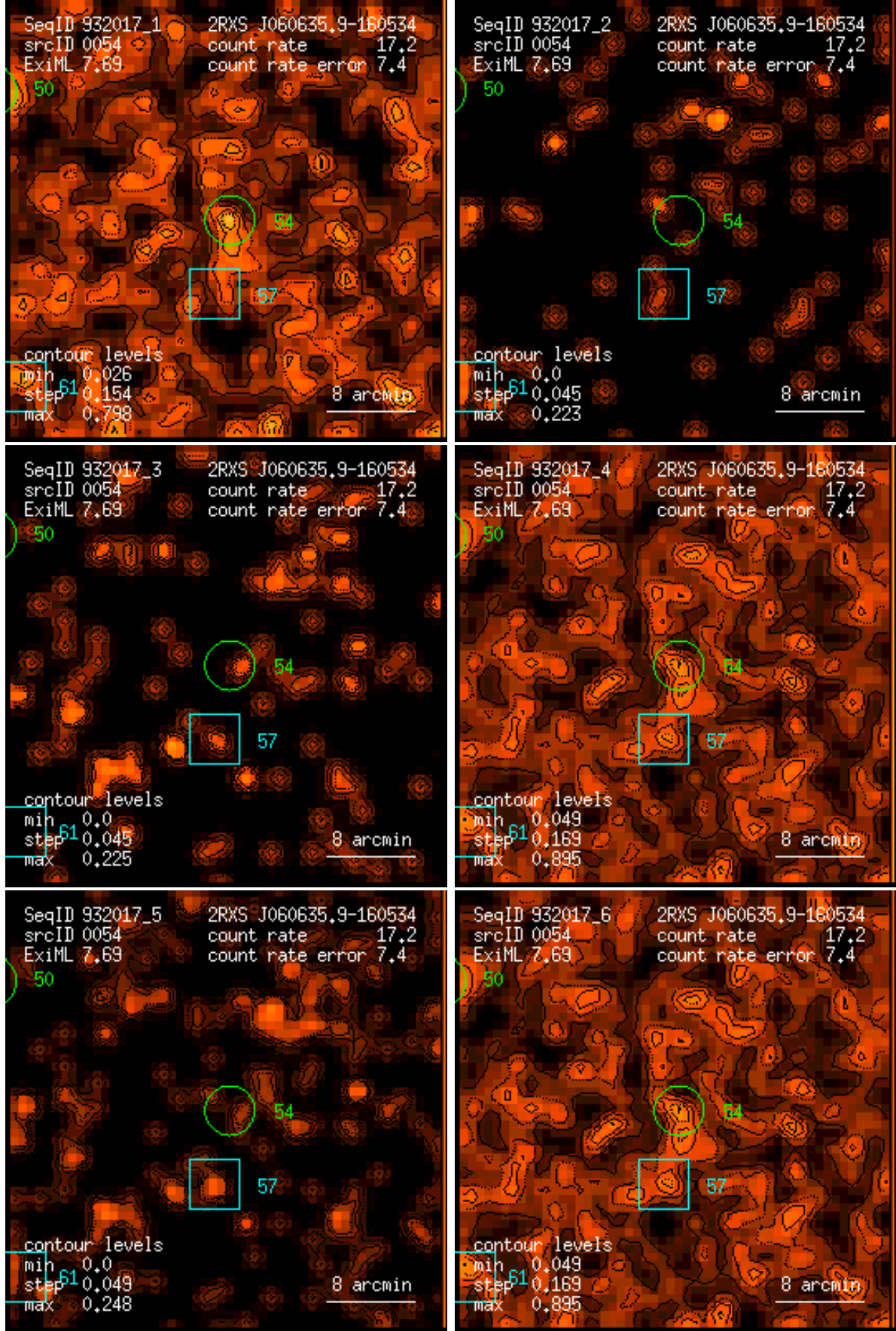
Figure 54: RASS 932017: detection 0054: band rate images, Gaussian filter: (1) PSPC channels 11 – 41, (2) 52 – 90, (3) 91 – 201, (4) 11 – 235, (5) 52 – 201, (6) 11 – 201. Broad band rates in counts/ks. Band rate contour levels in counts/ks/arcmin 2 .
