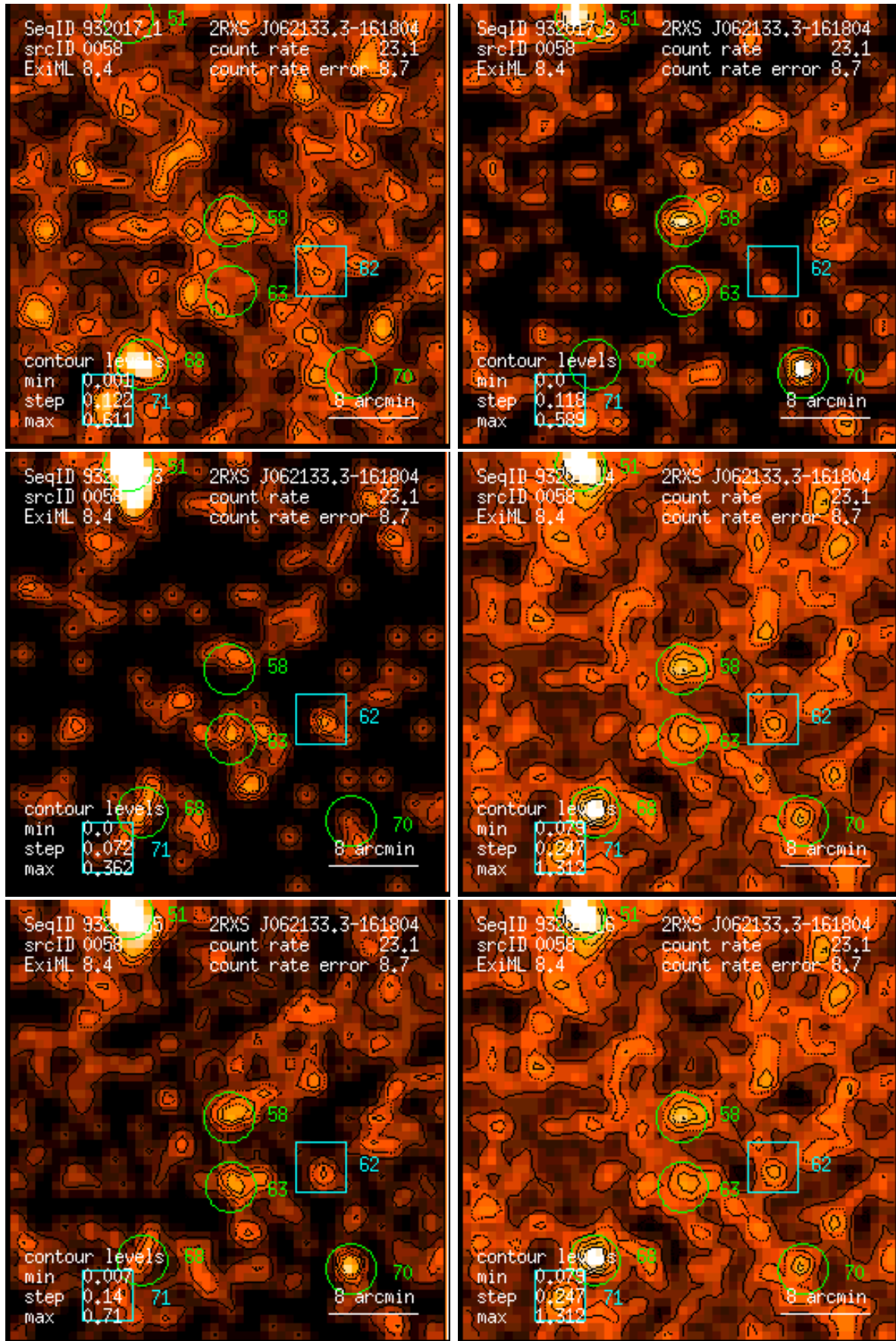
Figure 58: RASS 932017: detection 0058: band rate images, Gaussian filter: (1) PSPC channels 11 – 41, (2) 52 – 90, (3) 91 – 201, (4) 11 – 235, (5) 52 – 201, (6) 11 – 201. Broad band rates in counts/ks. Band rate contour levels in counts/ks/arcmin 2 .
