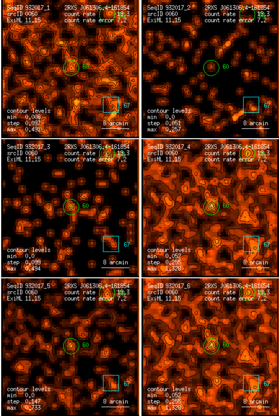
Figure 60: RASS 932017: detection 0060: band rate images, Gaussian filter: (1) PSPC channels 11 – 41, (2) 52 – 90, (3) 91 – 201, (4) 11 – 235, (5) 52 – 201, (6) 11 – 201. Broad band rates in counts/ks. Band rate contour levels in counts/ks/arcmin 2 .
