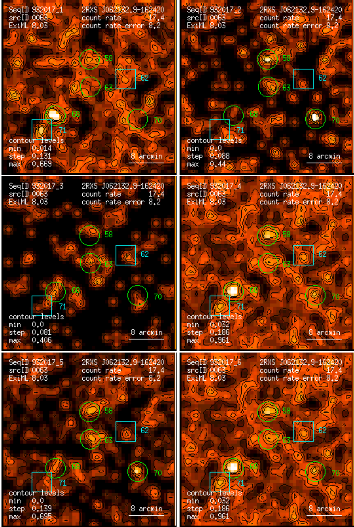
Figure 63: RASS 932017: detection 0063: band rate images, Gaussian filter: (1) PSPC channels 11 – 41, (2) 52 – 90, (3) 91 – 201, (4) 11 – 235, (5) 52 – 201, (6) 11 – 201. Broad band rates in counts/ks. Band rate contour levels in counts/ks/arcmin 2 .
