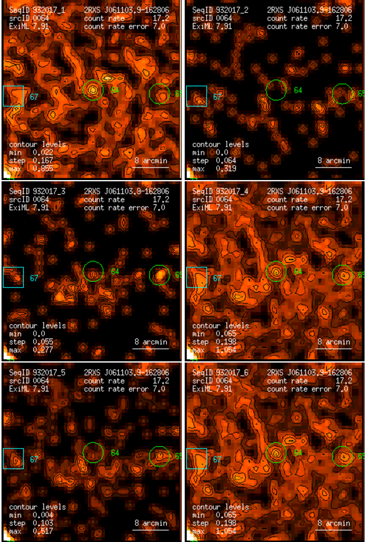
Figure 64: RASS 932017: detection 0064: band rate images, Gaussian filter: (1) PSPC channels 11 – 41, (2) 52 – 90, (3) 91 – 201, (4) 11 – 235, (5) 52 – 201, (6) 11 – 201. Broad band rates in counts/ks. Band rate contour levels in counts/ks/arcmin 2 .
