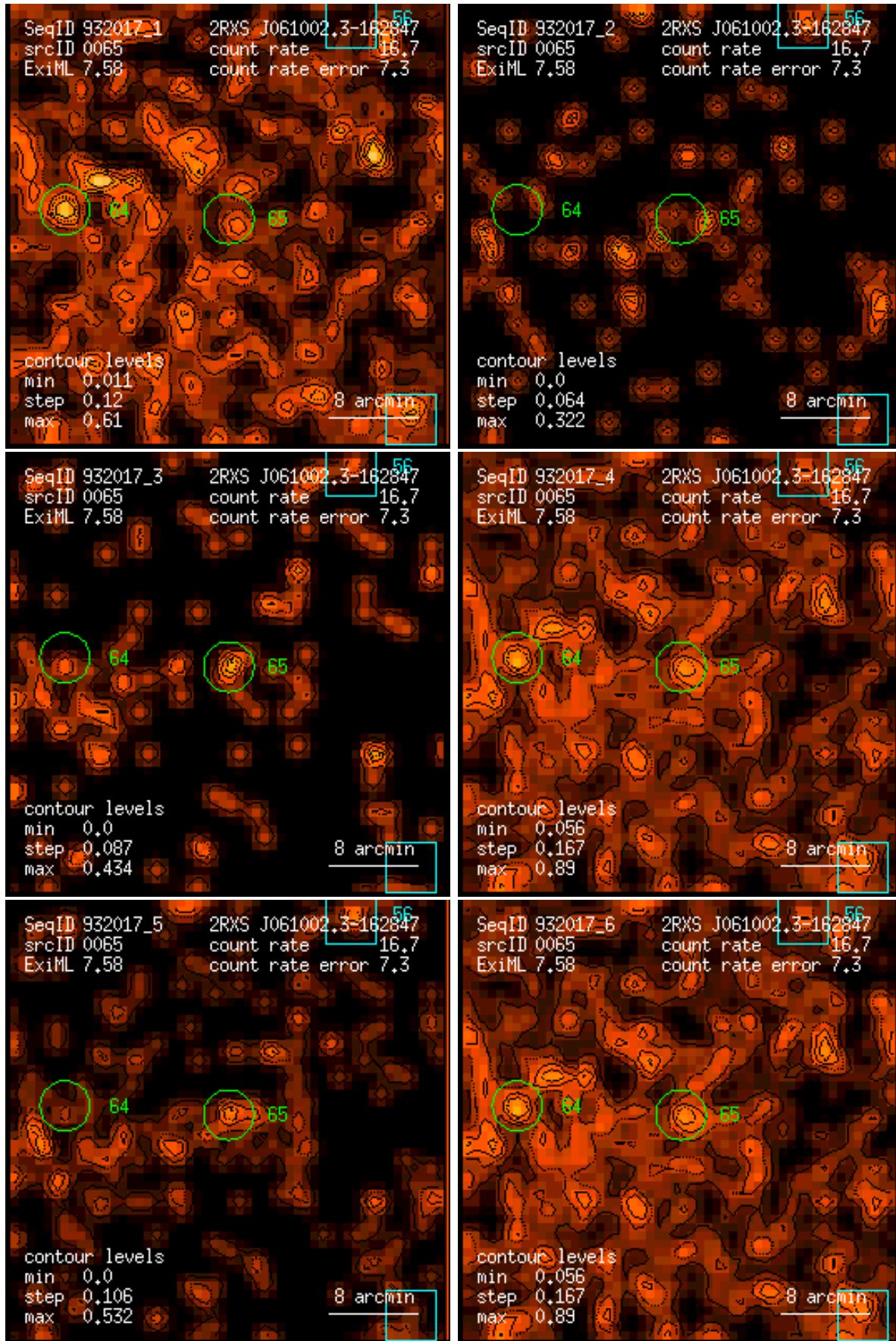
Figure 65: RASS 932017: detection 0065: band rate images, Gaussian filter: (1) PSPC channels 11 – 41, (2) 52 – 90, (3) 91 – 201, (4) 11 – 235, (5) 52 – 201, (6) 11 – 201. Broad band rates in counts/ks. Band rate contour levels in counts/ks/arcmin 2 .
