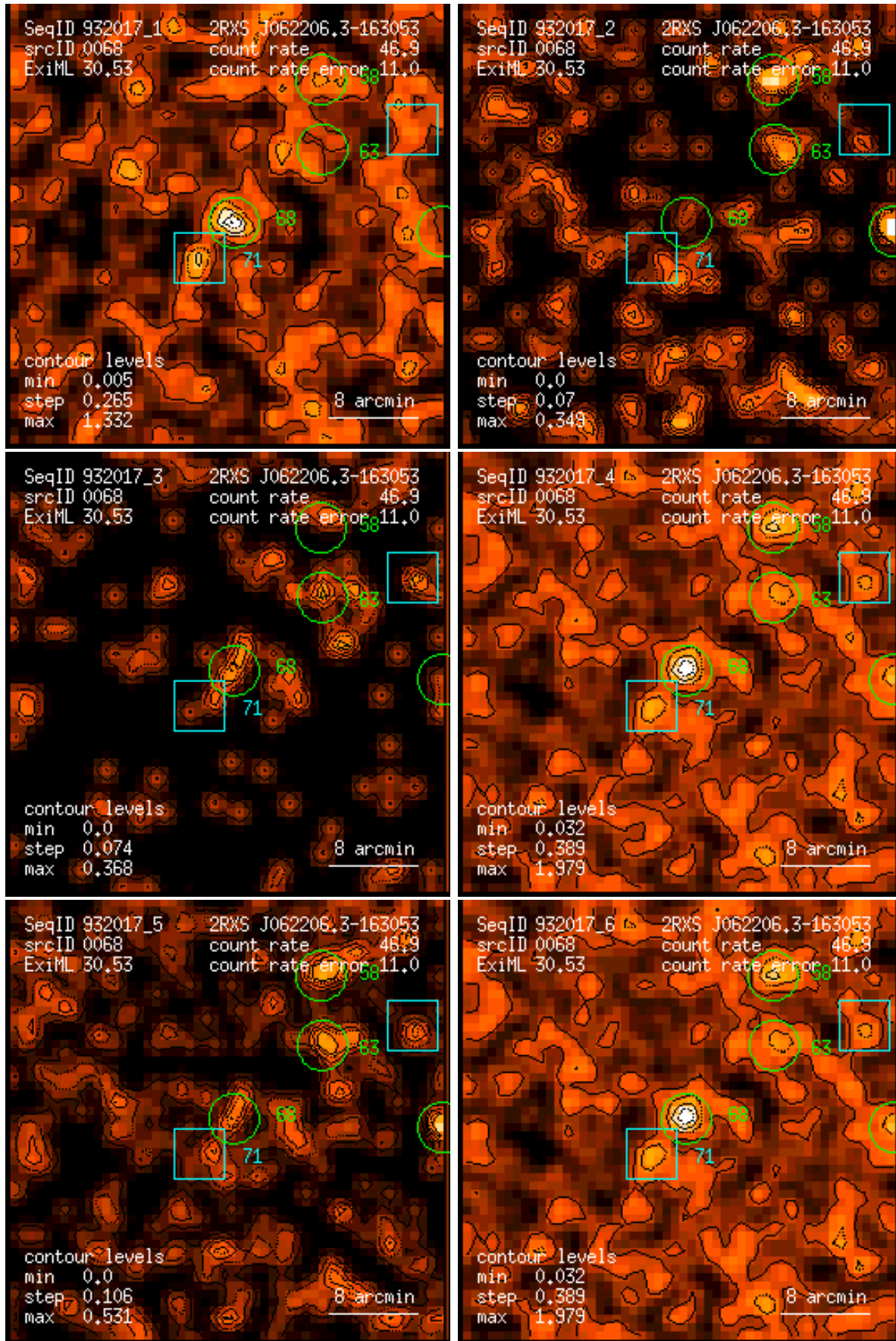
Figure 68: RASS 932017: detection 0068: band rate images, Gaussian filter: (1) PSPC channels 11 – 41, (2) 52 – 90, (3) 91 – 201, (4) 11 – 235, (5) 52 – 201, (6) 11 – 201. Broad band rates in counts/ks. Band rate contour levels in counts/ks/arcmin 2 .
