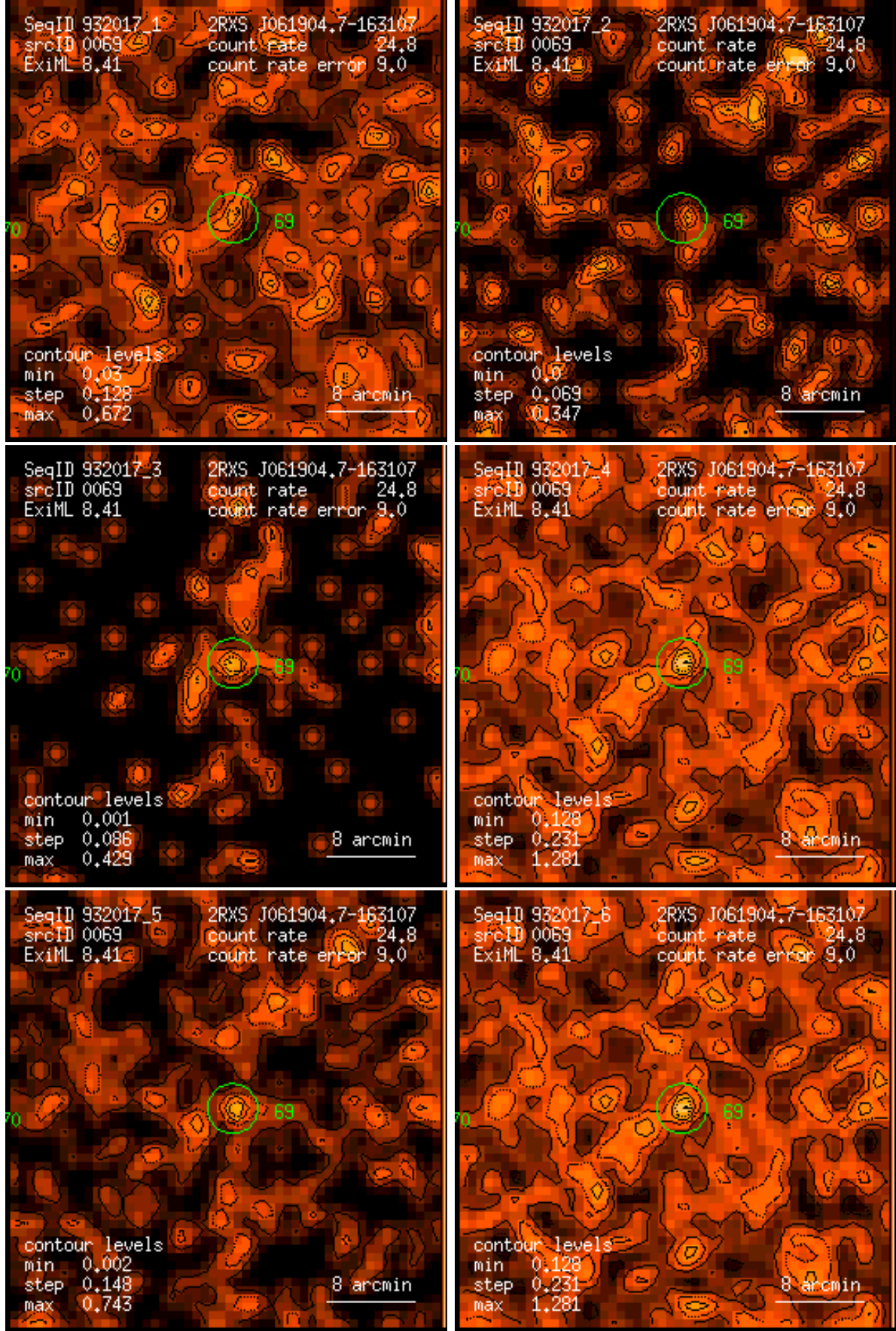
Figure 69: RASS 932017: detection 0069: band rate images, Gaussian filter: (1) PSPC channels 11 – 41, (2) 52 – 90, (3) 91 – 201, (4) 11 – 235, (5) 52 – 201, (6) 11 – 201. Broad band rates in counts/ks. Band rate contour levels in counts/ks/arcmin 2 .
