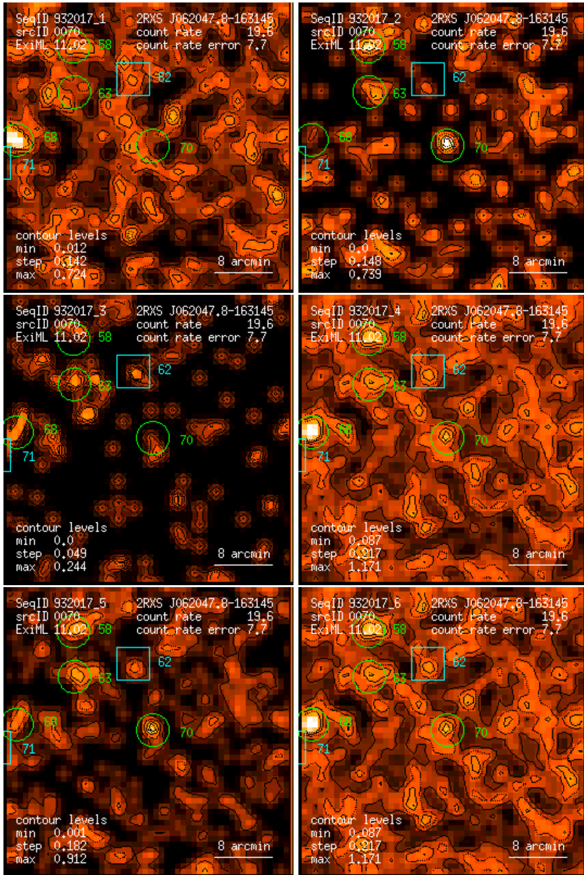
Figure 70: RASS 932017: detection 0070: band rate images, Gaussian filter: (1) PSPC channels 11 – 41, (2) 52 – 90, (3) 91 – 201, (4) 11 – 235, (5) 52 – 201, (6) 11 – 201. Broad band rates in counts/ks. Band rate contour levels in counts/ks/arcmin 2 .
