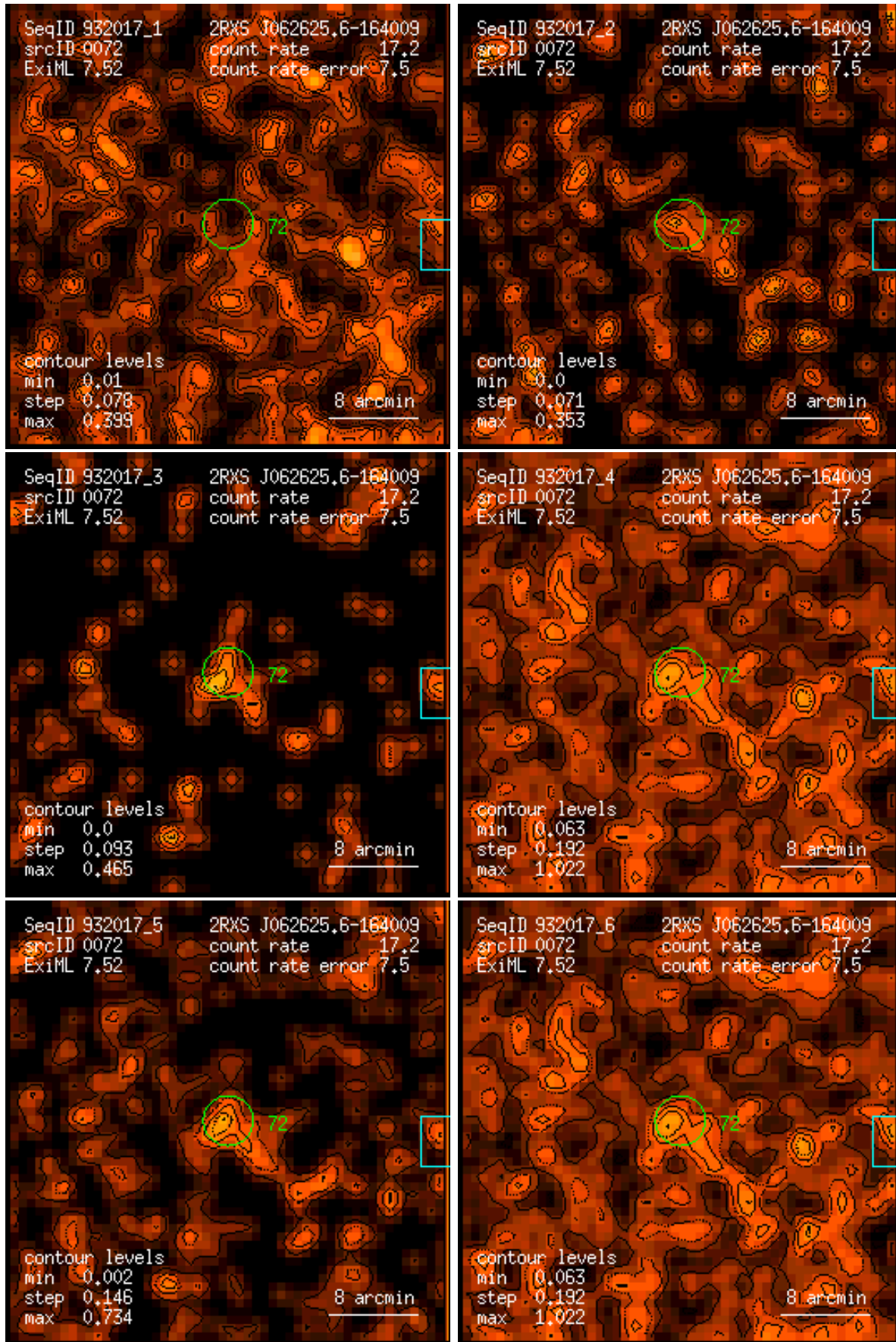
Figure 72: RASS 932017: detection 0072: band rate images, Gaussian filter: (1) PSPC channels 11 – 41, (2) 52 – 90, (3) 91 – 201, (4) 11 – 235, (5) 52 – 201, (6) 11 – 201. Broad band rates in counts/ks. Band rate contour levels in counts/ks/arcmin 2 .
