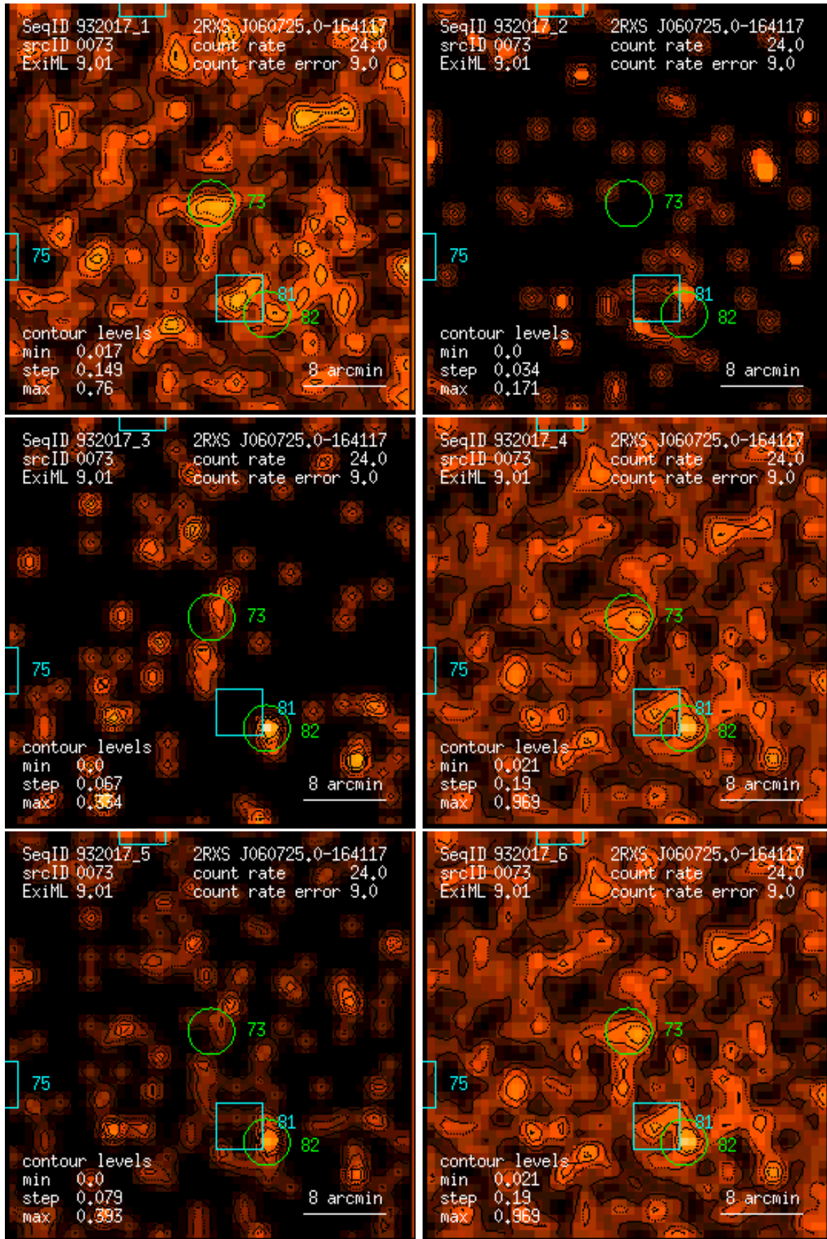
Figure 73: RASS 932017: detection 0073: band rate images, Gaussian filter: (1) PSPC channels 11 – 41, (2) 52 – 90, (3) 91 – 201, (4) 11 – 235, (5) 52 – 201, (6) 11 – 201. Broad band rates in counts/ks. Band rate contour levels in counts/ks/arcmin 2 .
