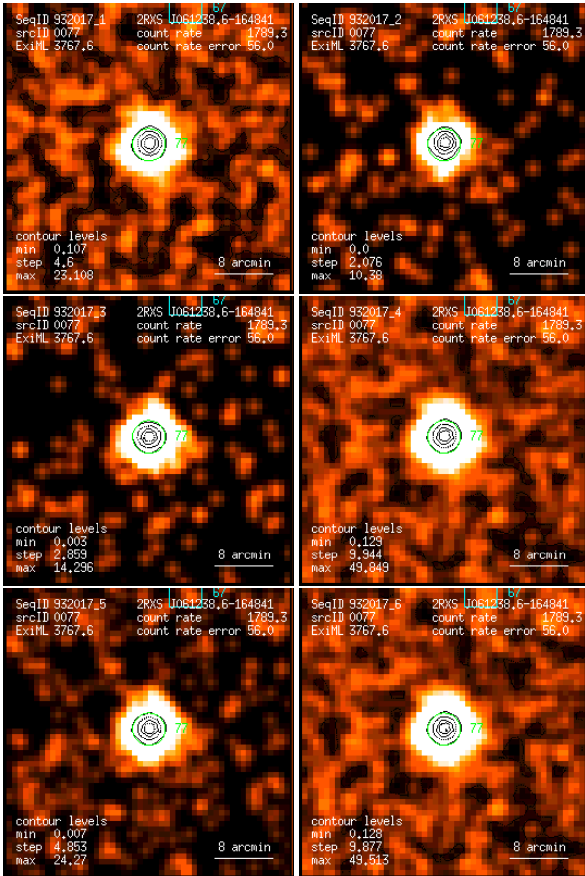
Figure 77: RASS 932017: detection 0077: band rate images, Gaussian filter: (1) PSPC channels 11 – 41, (2) 52 – 90, (3) 91 – 201, (4) 11 – 235, (5) 52 – 201, (6) 11 – 201. Broad band rates in counts/ks. Band rate contour levels in counts/ks/arcmin 2 .
