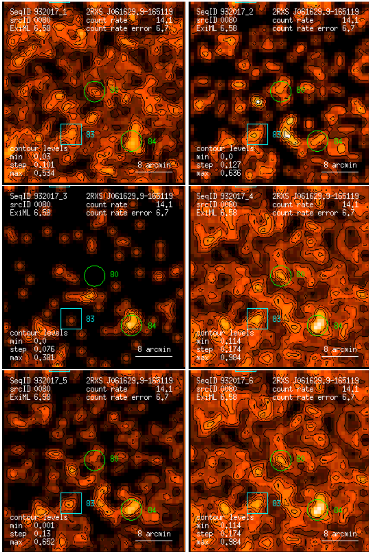
Figure 80: RASS 932017: detection 0080: band rate images, Gaussian filter: (1) PSPC channels 11 – 41, (2) 52 – 90, (3) 91 – 201, (4) 11 – 235, (5) 52 – 201, (6) 11 – 201. Broad band rates in counts/ks. Band rate contour levels in counts/ks/arcmin 2 .
