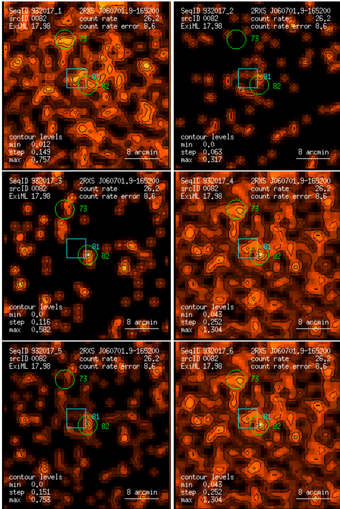
Figure 82: RASS 932017: detection 0082: band rate images, Gaussian filter: (1) PSPC channels 11 – 41, (2) 52 – 90, (3) 91 – 201, (4) 11 – 235, (5) 52 – 201, (6) 11 – 201. Broad band rates in counts/ks. Band rate contour levels in counts/ks/arcmin 2 .
