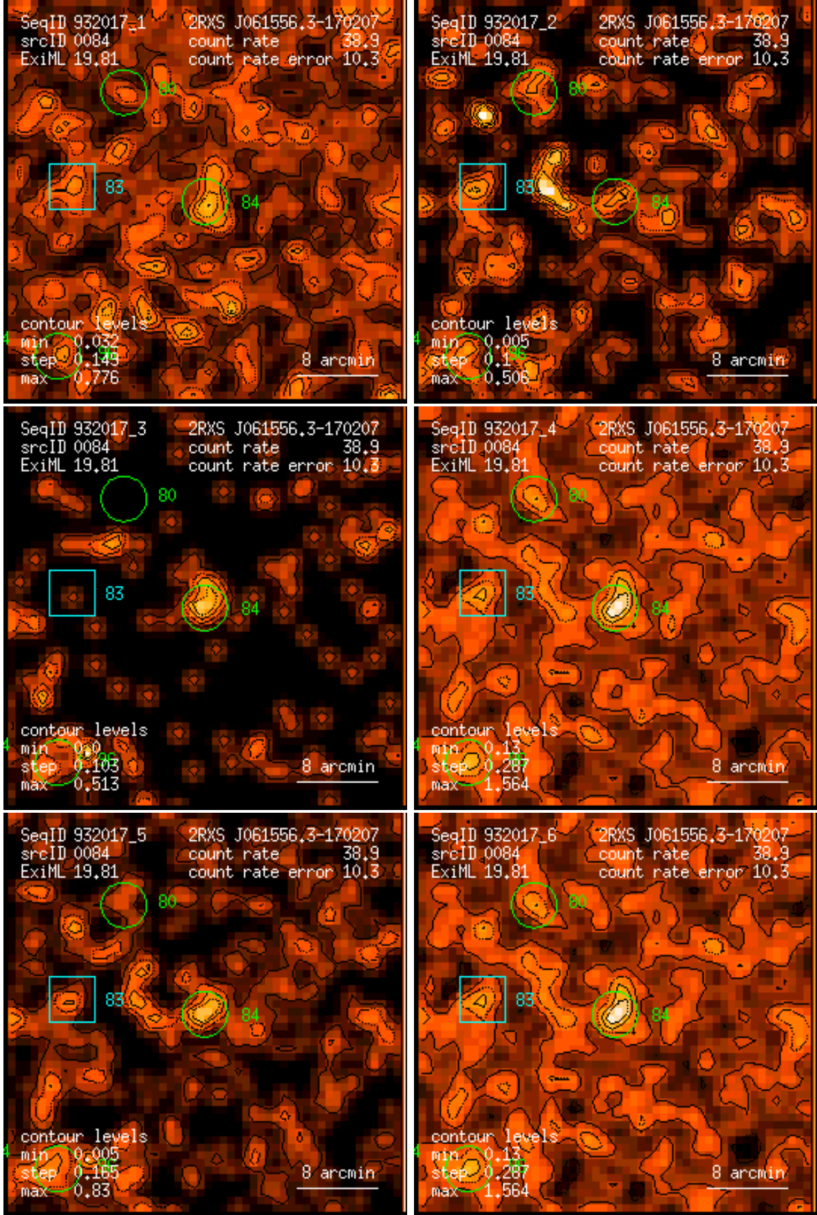
Figure 84: RASS 932017: detection 0084: band rate images, Gaussian filter: (1) PSPC channels 11 – 41, (2) 52 – 90, (3) 91 – 201, (4) 11 – 235, (5) 52 – 201, (6) 11 – 201. Broad band rates in counts/ks. Band rate contour levels in counts/ks/arcmin 2 .
