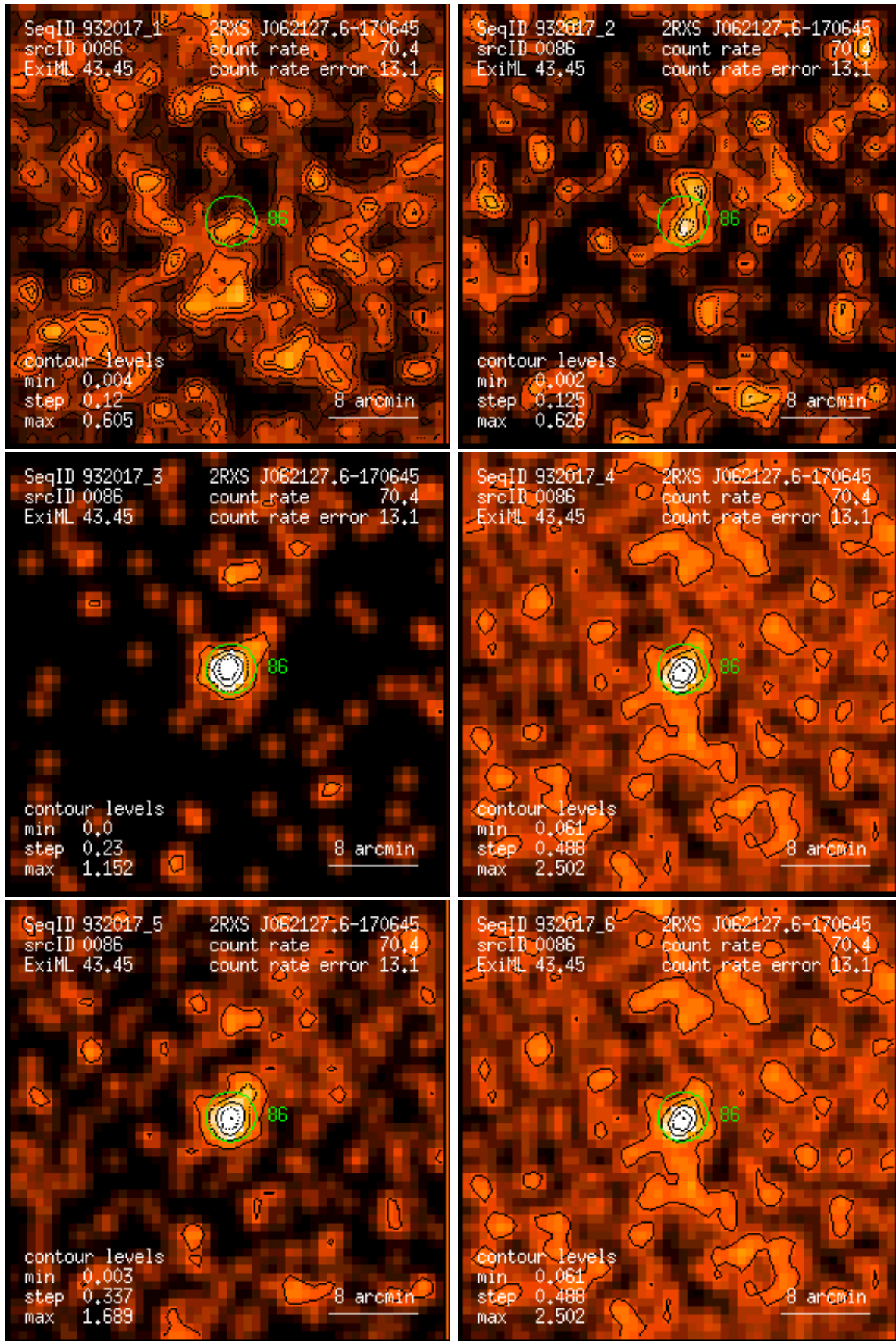
Figure 86: RASS 932017: detection 0086: band rate images, Gaussian filter: (1) PSPC channels 11 – 41, (2) 52 – 90, (3) 91 – 201, (4) 11 – 235, (5) 52 – 201, (6) 11 – 201. Broad band rates in counts/ks. Band rate contour levels in counts/ks/arcmin 2 .
