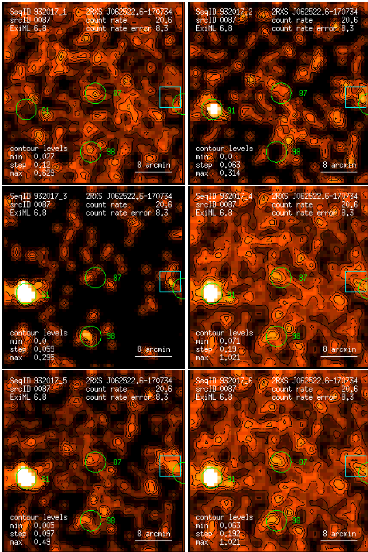
Figure 87: RASS 932017: detection 0087: band rate images, Gaussian filter: (1) PSPC channels 11 – 41, (2) 52 – 90, (3) 91 – 201, (4) 11 – 235, (5) 52 – 201, (6) 11 – 201. Broad band rates in counts/ks. Band rate contour levels in counts/ks/arcmin 2 .
