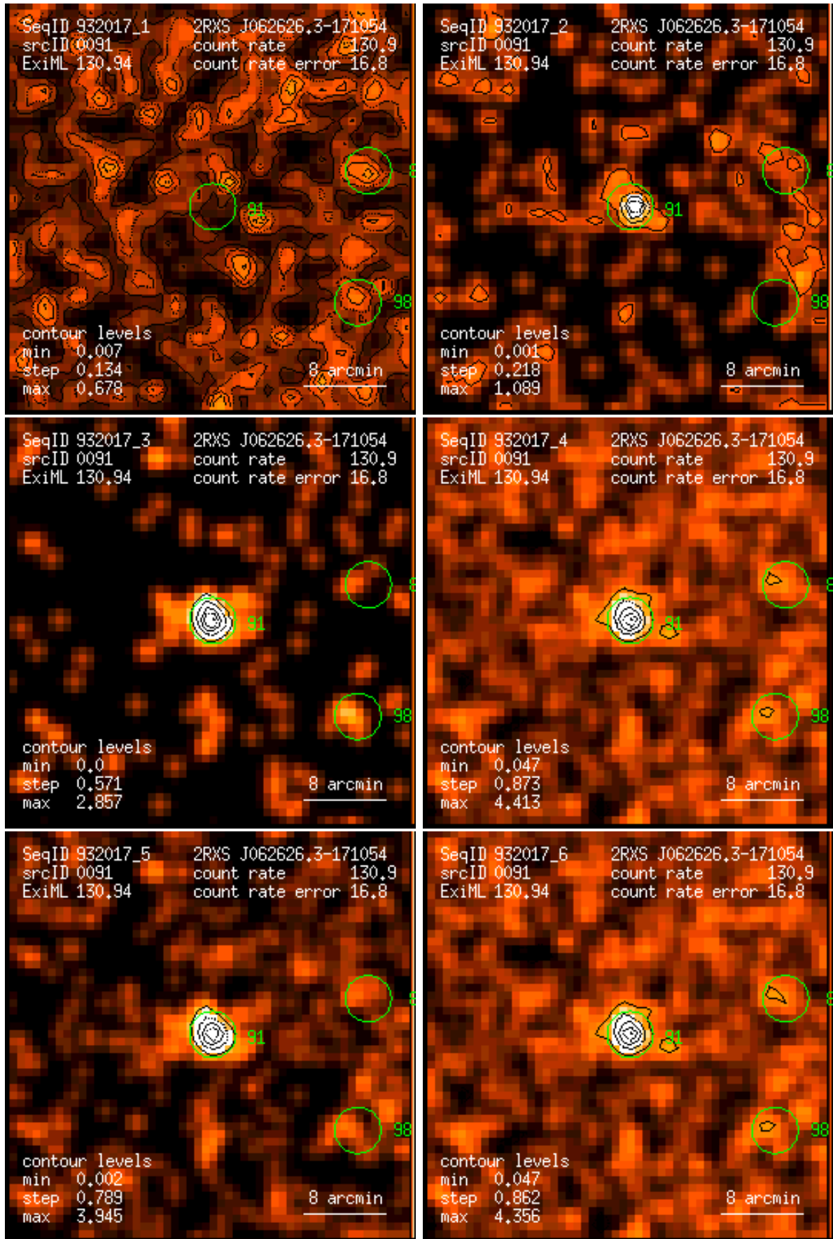
Figure 91: RASS 932017: detection 0091: band rate images, Gaussian filter: (1) PSPC channels 11 – 41, (2) 52 – 90, (3) 91 – 201, (4) 11 – 235, (5) 52 – 201, (6) 11 – 201. Broad band rates in counts/ks. Band rate contour levels in counts/ks/arcmin 2 .
