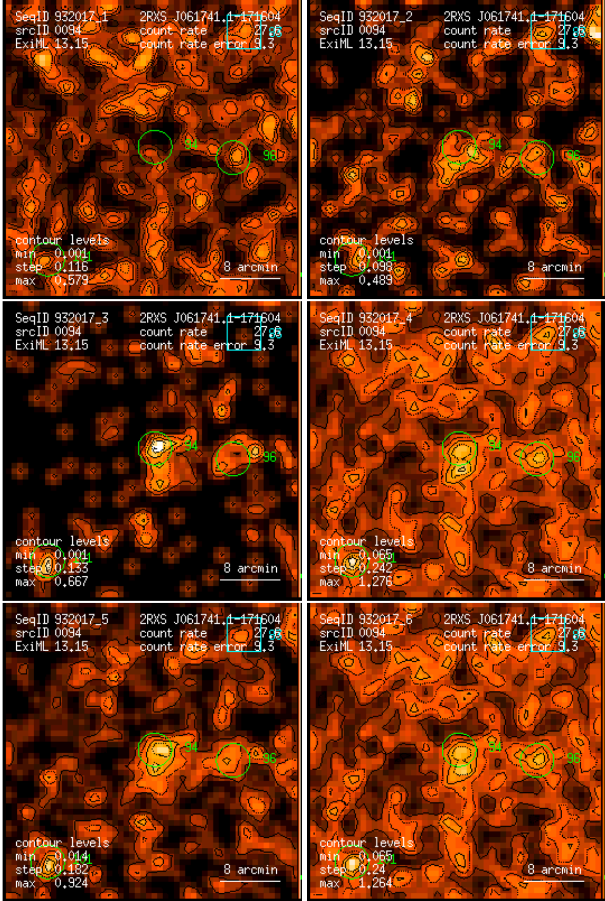
Figure 94: RASS 932017: detection 0094: band rate images, Gaussian filter: (1) PSPC channels 11 – 41, (2) 52 – 90, (3) 91 – 201, (4) 11 – 235, (5) 52 – 201, (6) 11 – 201. Broad band rates in counts/ks. Band rate contour levels in counts/ks/arcmin 2 .
