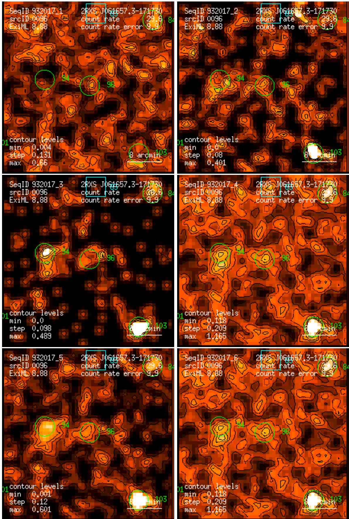
Figure 96: RASS 932017: detection 0096: band rate images, Gaussian filter: (1) PSPC channels 11 – 41, (2) 52 – 90, (3) 91 – 201, (4) 11 – 235, (5) 52 – 201, (6) 11 – 201. Broad band rates in counts/ks. Band rate contour levels in counts/ks/arcmin 2 .
