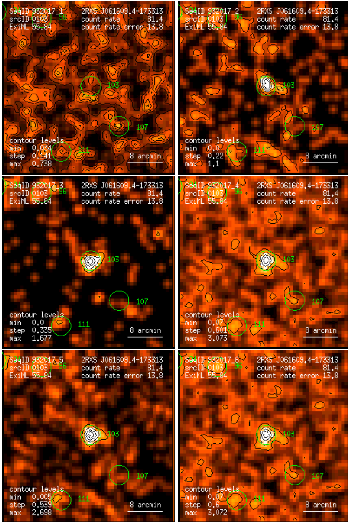
Figure 103: RASS 932017: detection 0103: band rate images, Gaussian filter: (1) PSPC channels 11 – 41, (2) 52 – 90, (3) 91 – 201, (4) 11 – 235, (5) 52 – 201, (6) 11 – 201. Broad band rates in counts/ks. Band rate contour levels in counts/ks/arcmin 2 .
