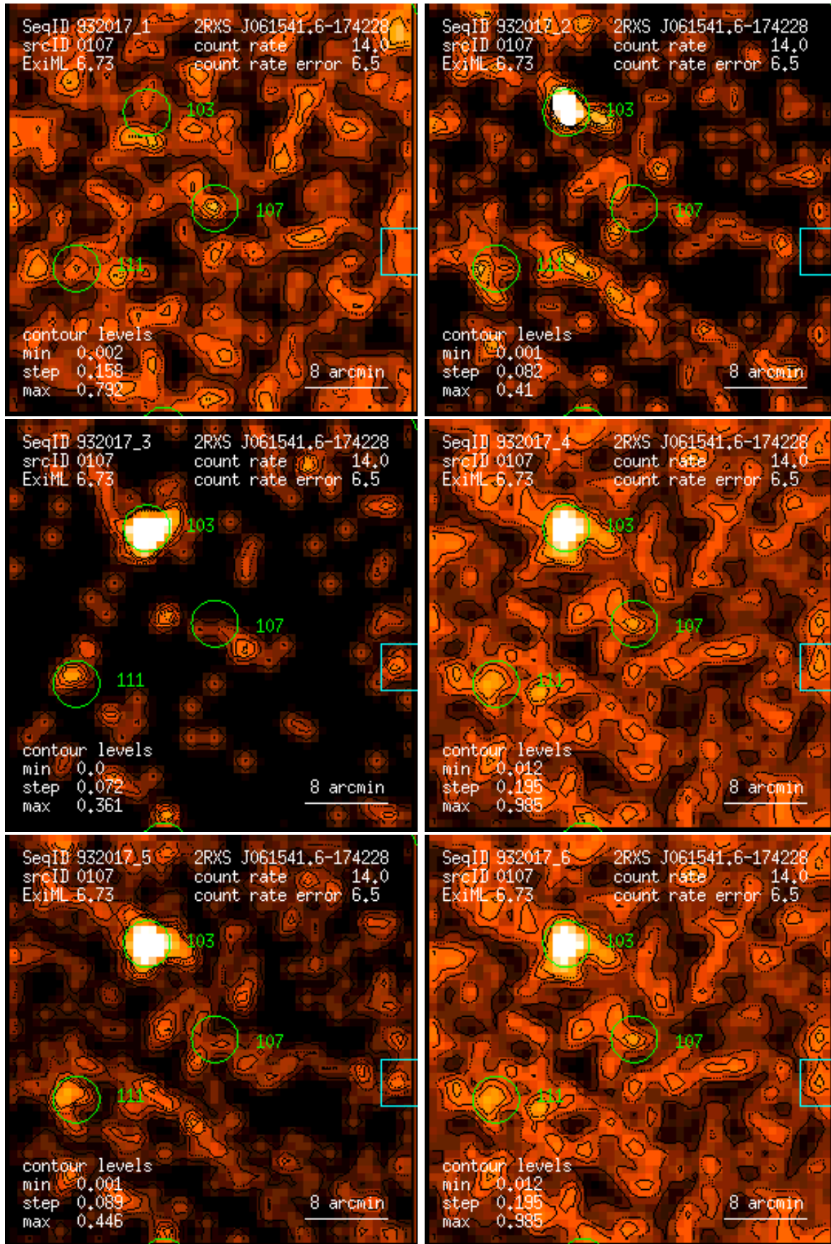
Figure 107: RASS 932017: detection 0107: band rate images, Gaussian filter: (1) PSPC channels 11 – 41, (2) 52 – 90, (3) 91 – 201, (4) 11 – 235, (5) 52 – 201, (6) 11 – 201. Broad band rates in counts/ks. Band rate contour levels in counts/ks/arcmin 2 .
