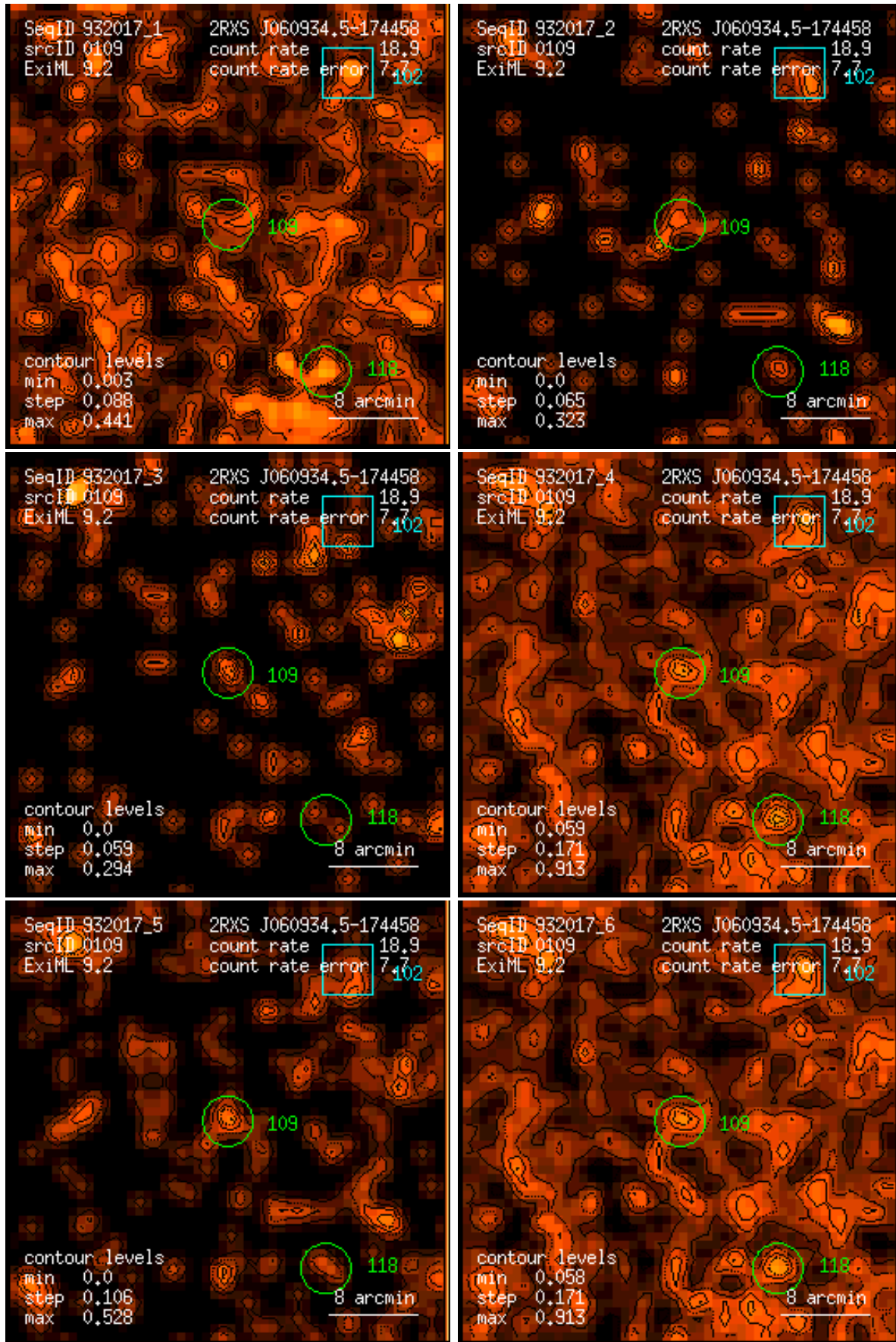
Figure 109: RASS 932017: detection 0109: band rate images, Gaussian filter: (1) PSPC channels 11 – 41, (2) 52 – 90, (3) 91 – 201, (4) 11 – 235, (5) 52 – 201, (6) 11 – 201. Broad band rates in counts/ks. Band rate contour levels in counts/ks/arcmin 2 .
