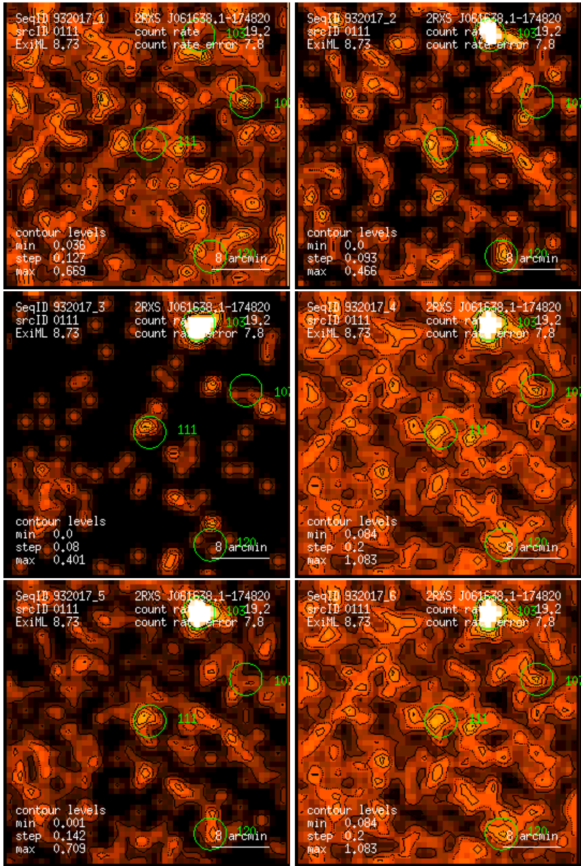
Figure 111: RASS 932017: detection 0111: band rate images, Gaussian filter: (1) PSPC channels 11 – 41, (2) 52 – 90, (3) 91 – 201, (4) 11 – 235, (5) 52 – 201, (6) 11 – 201. Broad band rates in counts/ks. Band rate contour levels in counts/ks/arcmin 2 .
