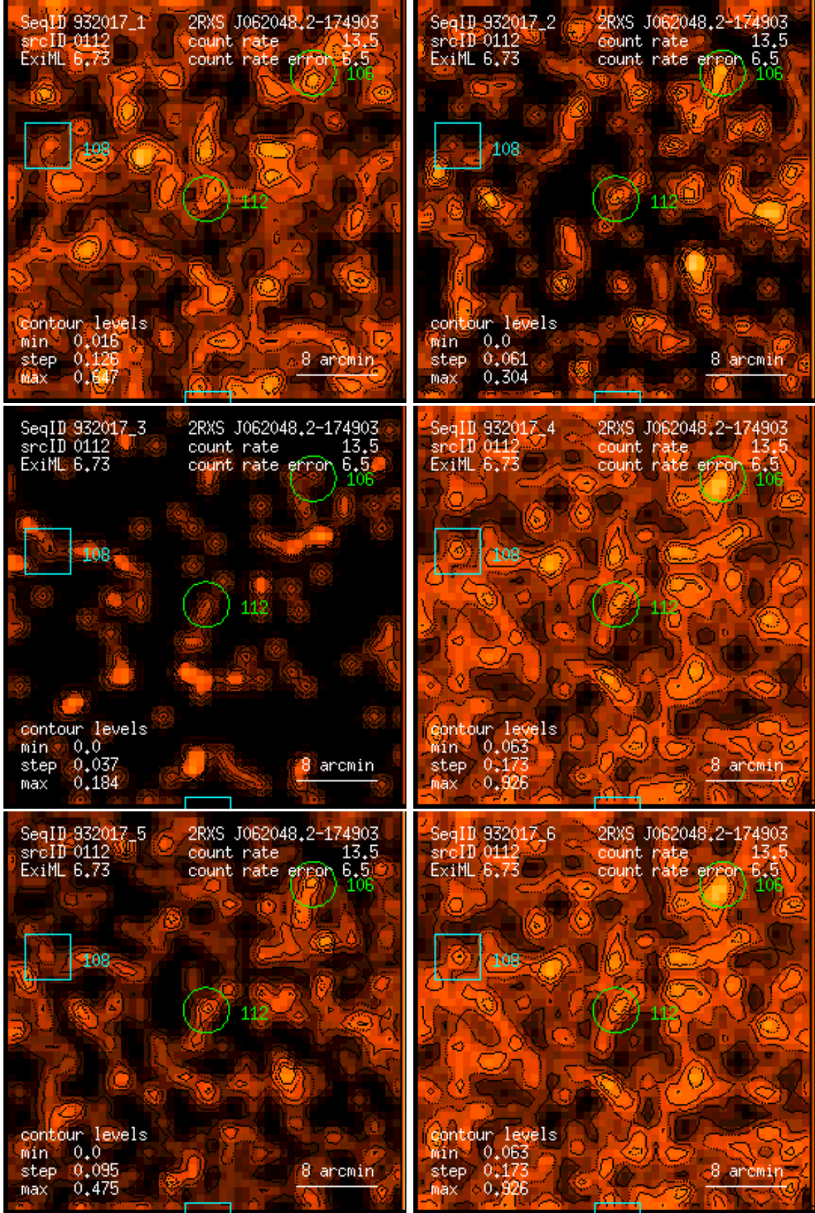
Figure 112: RASS 932017: detection 0112: band rate images, Gaussian filter: (1) PSPC channels 11 – 41, (2) 52 – 90, (3) 91 – 201, (4) 11 – 235, (5) 52 – 201, (6) 11 – 201. Broad band rates in counts/ks. Band rate contour levels in counts/ks/arcmin 2 .
