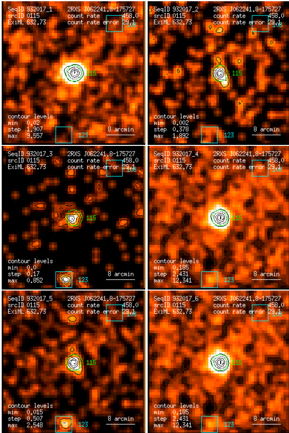
Figure 115: RASS 932017: detection 0115: band rate images, Gaussian filter: (1) PSPC channels 11 – 41, (2) 52 – 90, (3) 91 – 201, (4) 11 – 235, (5) 52 – 201, (6) 11 – 201. Broad band rates in counts/ks. Band rate contour levels in counts/ks/arcmin 2 .
