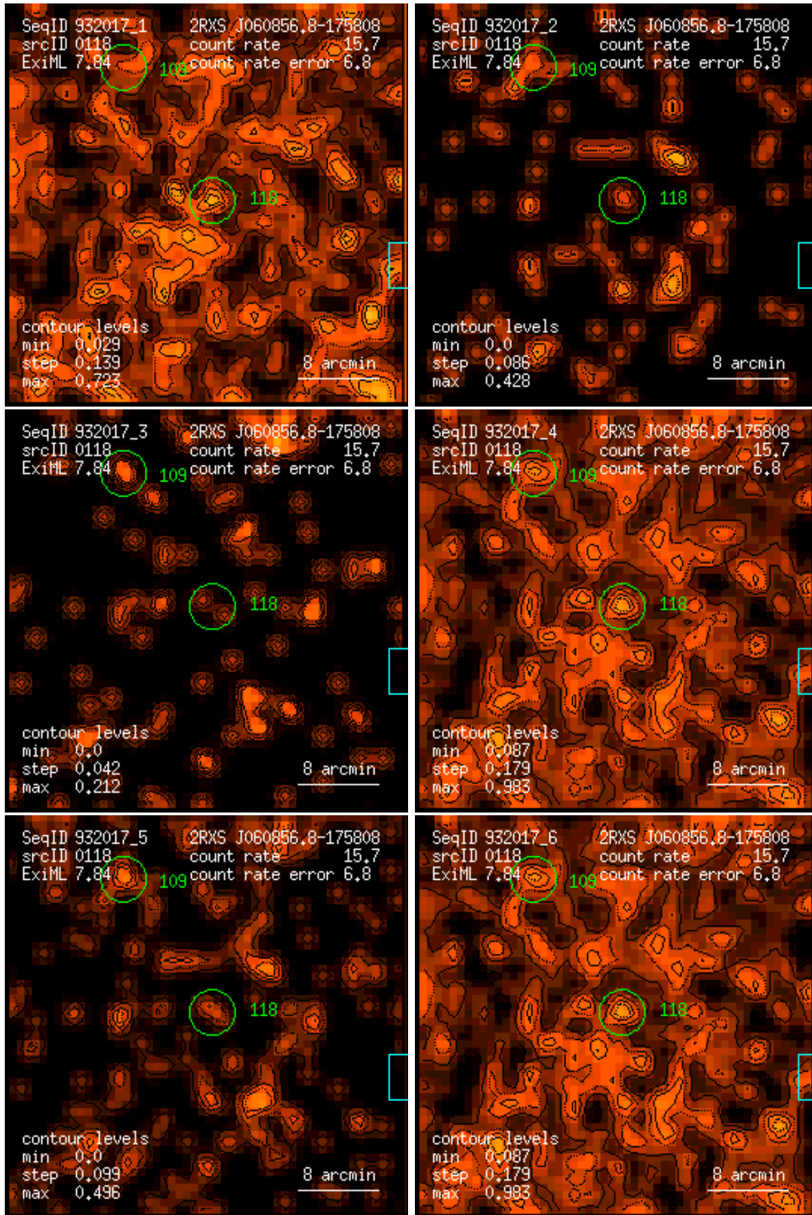
Figure 118: RASS 932017: detection 0118: band rate images, Gaussian filter: (1) PSPC channels 11 – 41, (2) 52 – 90, (3) 91 – 201, (4) 11 – 235, (5) 52 – 201, (6) 11 – 201. Broad band rates in counts/ks. Band rate contour levels in counts/ks/arcmin 2 .
