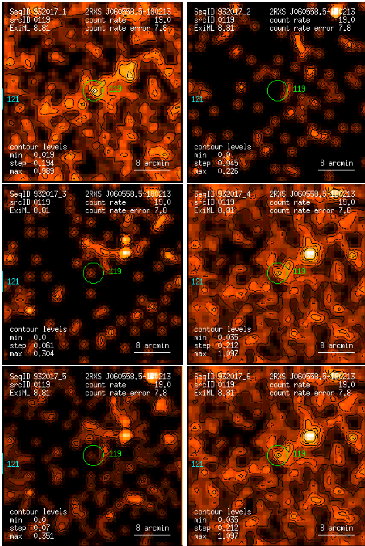
Figure 119: RASS 932017: detection 0119: band rate images, Gaussian filter: (1) PSPC channels 11 – 41, (2) 52 – 90, (3) 91 – 201, (4) 11 – 235, (5) 52 – 201, (6) 11 – 201. Broad band rates in counts/ks. Band rate contour levels in counts/ks/arcmin 2 .
