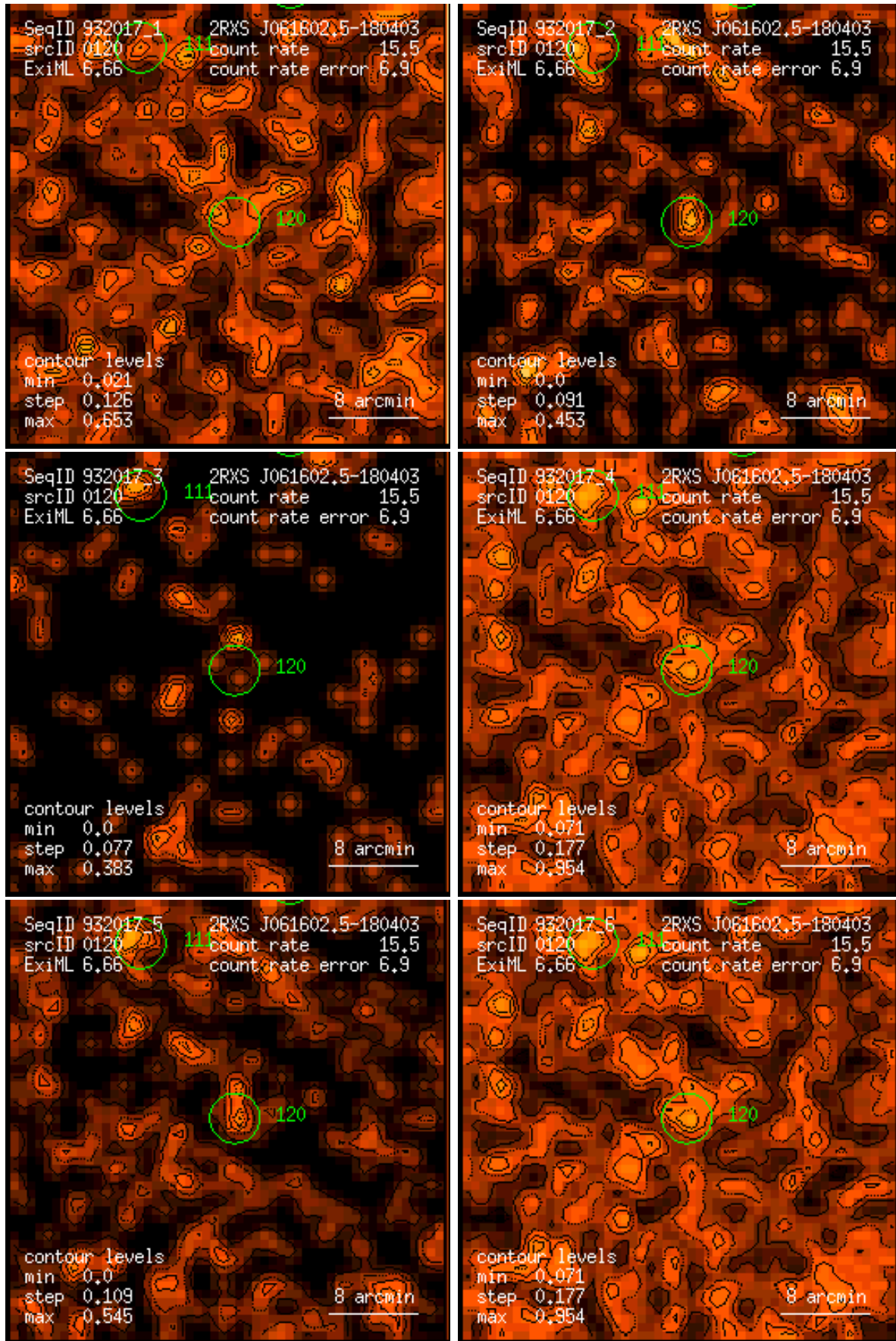
Figure 120: RASS 932017: detection 0120: band rate images, Gaussian filter: (1) PSPC channels 11 – 41, (2) 52 – 90, (3) 91 – 201, (4) 11 – 235, (5) 52 – 201, (6) 11 – 201. Broad band rates in counts/ks. Band rate contour levels in counts/ks/arcmin 2 .
