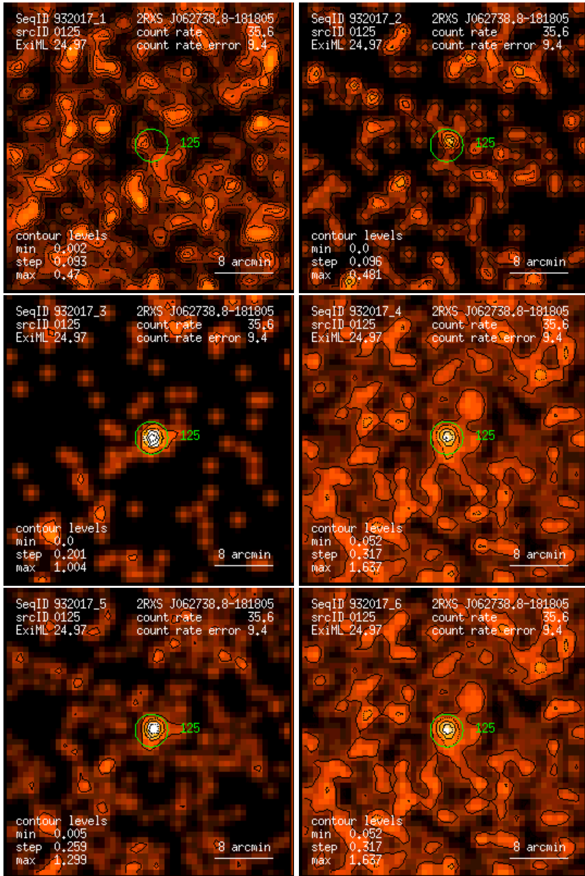
Figure 125: RASS 932017: detection 0125: band rate images, Gaussian filter: (1) PSPC channels 11 – 41, (2) 52 – 90, (3) 91 – 201, (4) 11 – 235, (5) 52 – 201, (6) 11 – 201. Broad band rates in counts/ks. Band rate contour levels in counts/ks/arcmin 2 .
