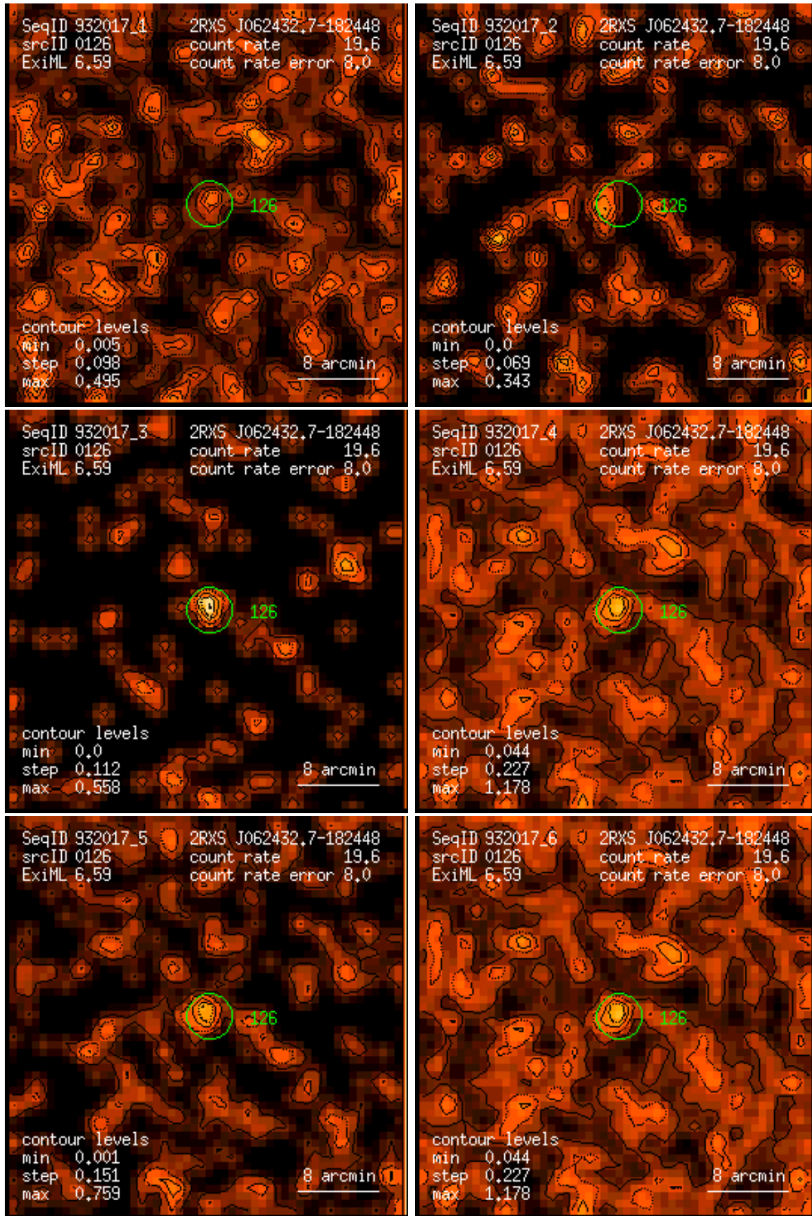
Figure 126: RASS 932017: detection 0126: band rate images, Gaussian filter: (1) PSPC channels 11 – 41, (2) 52 – 90, (3) 91 – 201, (4) 11 – 235, (5) 52 – 201, (6) 11 – 201. Broad band rates in counts/ks. Band rate contour levels in counts/ks/arcmin 2 .
