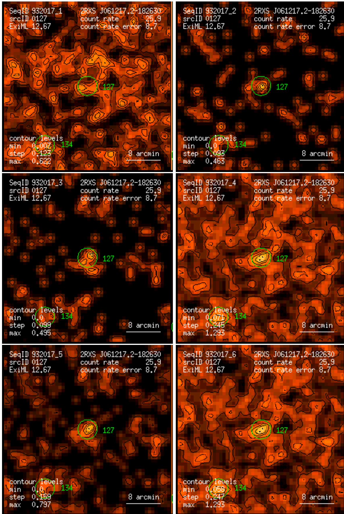
Figure 127: RASS 932017: detection 0127: band rate images, Gaussian filter: (1) PSPC channels 11 – 41, (2) 52 – 90, (3) 91 – 201, (4) 11 – 235, (5) 52 – 201, (6) 11 – 201. Broad band rates in counts/ks. Band rate contour levels in counts/ks/arcmin 2 .
