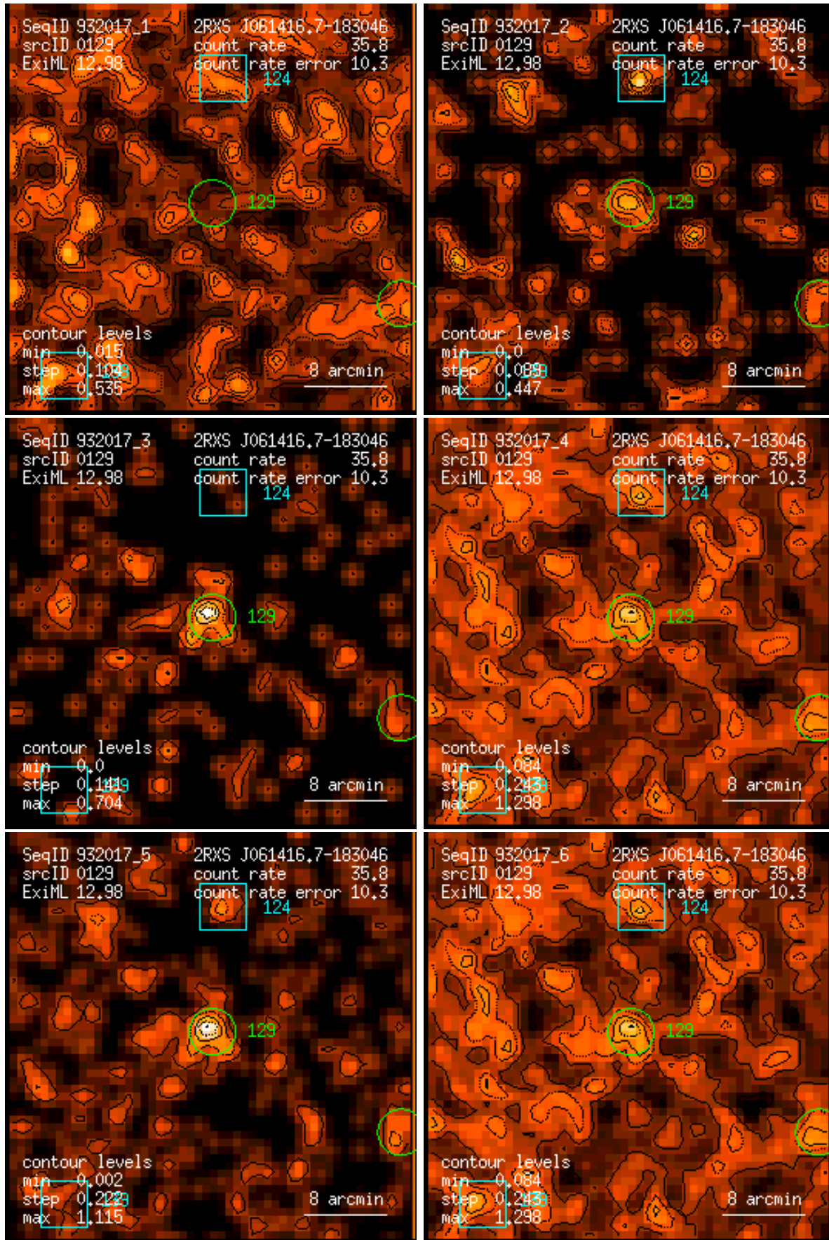
Figure 129: RASS 932017: detection 0129: band rate images, Gaussian filter: (1) PSPC channels 11 – 41, (2) 52 – 90, (3) 91 – 201, (4) 11 – 235, (5) 52 – 201, (6) 11 – 201. Broad band rates in counts/ks. Band rate contour levels in counts/ks/arcmin 2 .
